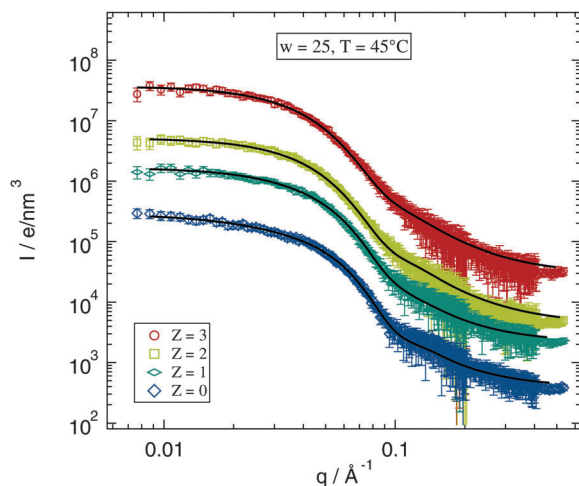
Fig. 5 Scattering curves for w = 25 and T = 45\text{ }^{\circ}\text{C} with different number Z of polymer chains per droplet. Solid lines are fits of the model described in Section 2.2.2. Curves are shifted vertically for clarity.
