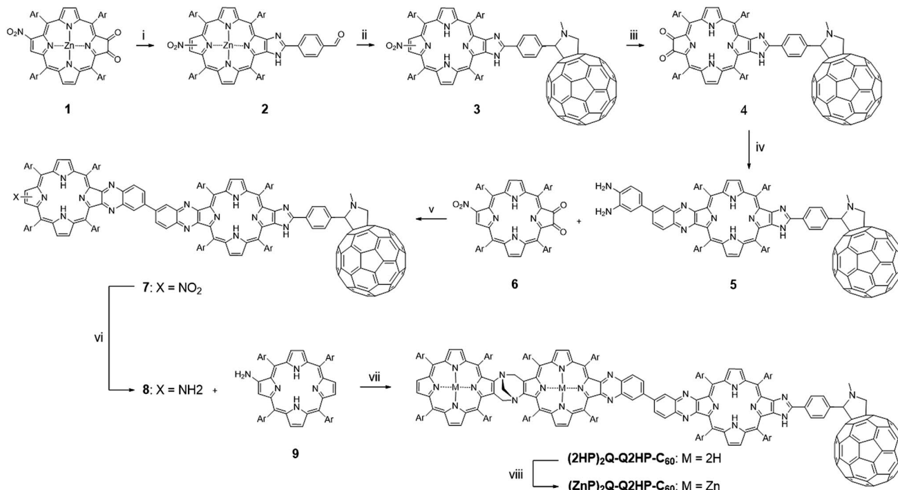
Scheme 1 Reagents and conditions: (i) terephthalaldehyde, NH_4OAc , CHCl_3 , reflux (90%); (ii) 1, CH_2Cl_2 , HCl, stir (89%); 2, fullerene, N -methylglycine, toluene, reflux (75%); (iii) 1, SnCl_2 \cdot 2H_2O , HCl/ Et_2O , stir; 2, CH_2Cl_2 , photooxidation (54%); (iv) 3,3'-diaminobenzidine, CH_2Cl_2 , stir (80%); (v) CH_2Cl_2 , stir (56%); (vi) SnCl_2 \cdot 2H_2O , HCl, CH_2Cl_2 , stir; (vii) THF, HCl/ EtOH , formaldehyde, stir, 70 °C (16%); (viii) Zn(OAc)_2 \cdot 2H_2O , CH_2Cl_2 / MeOH , stir (58%). Ar = 3,5-di- tert -butylphenyl.
