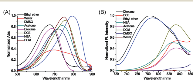
Fig. 1 The normalized absorption and fluorescence spectra of MCY-BF 2 (10 \mu\text{M} ) in eight solvents with different polarity. The excitation wavelength is 700 nm.
