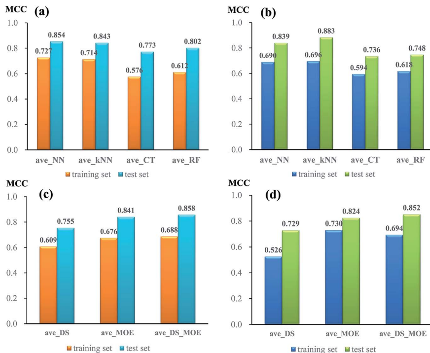
Fig. 3 The comparison of average MCC values made by different algorithms (a and b) and different sets of descriptors (c and d) against glutamate-induced neurotoxicity (a and c) and H_2O_2 -induced neurotoxicity (b and d) on training set and test set.
