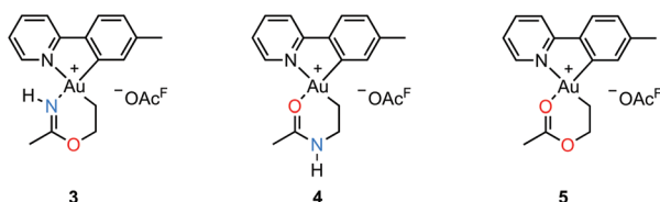
Scheme 3 Possible structures of the metallacyclic \text{Au}(\text{III}) complex.
