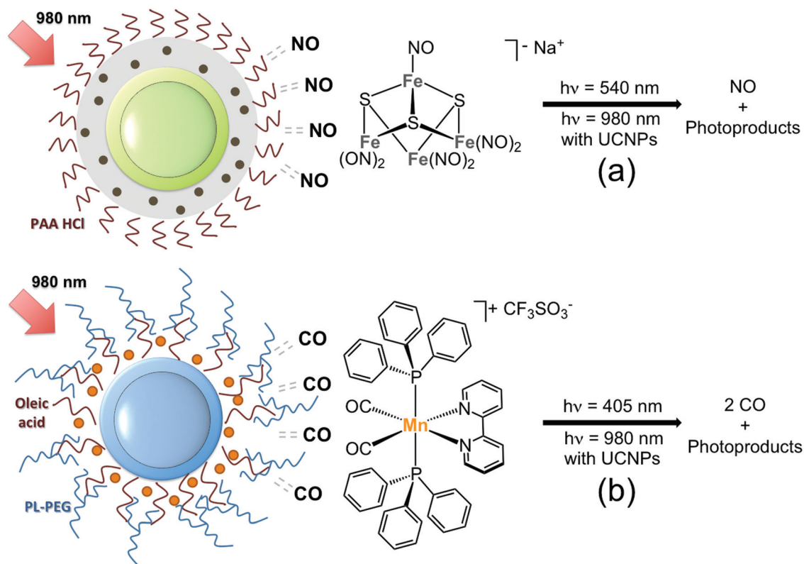
Fig. 3 Schematic representation of UCNPs nanocarriers for the NIR-light photorelease of (a) NO from RBS (●) and (b) CO from the complex cis,trans -[Mn(bpy)(CO) 2 (PPh 3 ) 2 ][CF 3 SO 3 ] - (●). Adapted from ref. 15 and 18.
