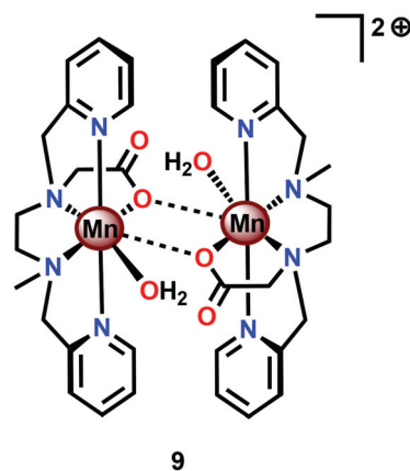
Fig. 7 Structure of the dimeric Mn II,II complex [Mn 2 II,II (mcbpen) 2 (OH 2 ) 2 ] 2+ (9).
