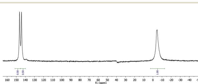
Fig. 4 ^{31}\text{P} NMR spectrum of supported phosphine–phosphite \text{L}_8 clearly showing the presence of both epimers in a 1 : 1 ratio.
