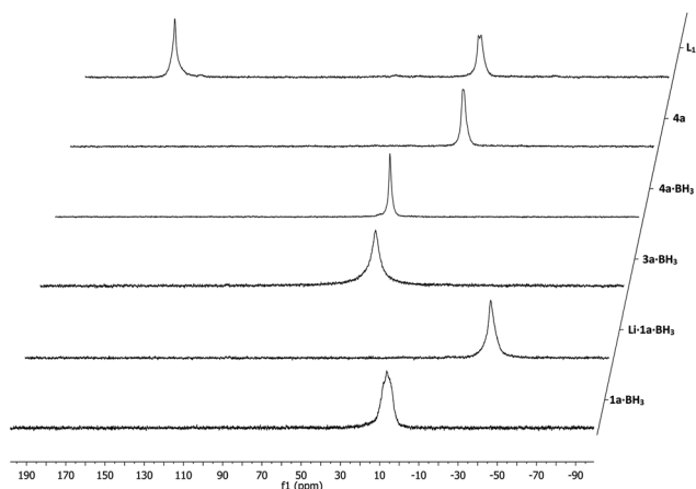
Fig. 2 Solid-phase synthesis of representative supported phosphine–phosphite \text{L}_1 as monitored by gel-phase ^{31}\text{P} NMR spectroscopy.
