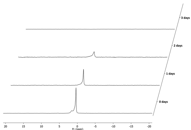
Fig. 3 Hydrolysis of representative supported phosphine–borane sulfate 3\text{a-BH}_3 monitored by ^7\text{Li} NMR spectroscopy.
