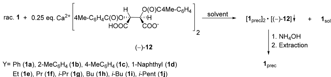
Scheme 13 General protocol for the resolution of 1-aryl- and 1-alkyl-3-methyl-3-phospholene 1-oxides ( 1a–j ) with \text{Ca}(\text{H-DPTTA})_2 [(-)\text{-}\mathbf{12}] .
