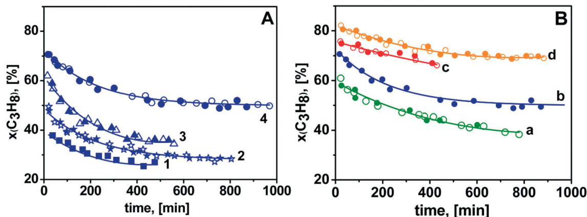
Fig. 6 C_3H_8 conversion vs. reaction time during ODH of propane on the Cr/DHS catalysts ( T = 873 K, w = 200 h -1 ) in the as-prepared state (open symbols) and after reaction and subsequent treatment in flowing O_2 at 873 K for 6 h (full symbols: after 5–8 runs). Panel A refers to the reaction performed using CO_2 as the oxidant ( C_3H_8 : CO_2 : N_2 = 15 : 30 : 55 ) on the catalyst: 1) 0.25-Cr/DHS, 2) 0.5-Cr/DHS, 3) 1.0-Cr/DHS, 4) 2.0-Cr/DHS. Panel B shows data obtained on the 2.0-Cr/DHS catalyst under different reaction conditions: a) C_3H_8 : N_2 = 15 : 85 (green curves; full symbols: after 5 runs); b) C_3H_8 : CO_2 : N_2 = 15 : 30 : 55 (blue curves; full symbols: after 8 runs); c) C_3H_8 : O_2 : N_2 = 15 : 3 : 82 (red curves; full symbols: after 5 runs); d) C_3H_8 : CO_2 : O_2 : N_2 = 15 : 30 : 3 : 52 (orange curves; full symbols: after 8 runs).
