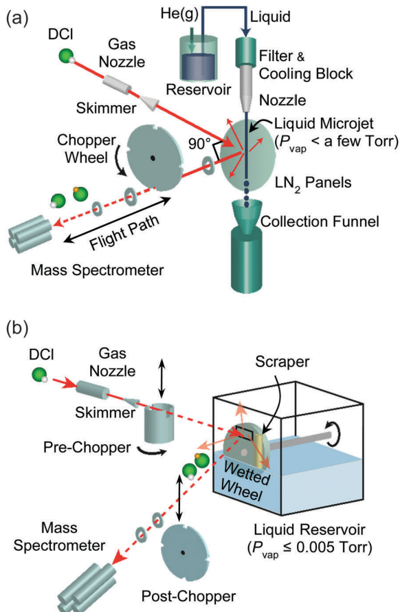
Fig. 3 Experimental setups used in our laboratory for molecular beam scattering experiments with (a) liquid microjets and (b) flat liquid films. The figure illustrates collisions of DCl that exit the liquids as DCl and \text{D} \rightarrow \text{H} exchanged HCl.
