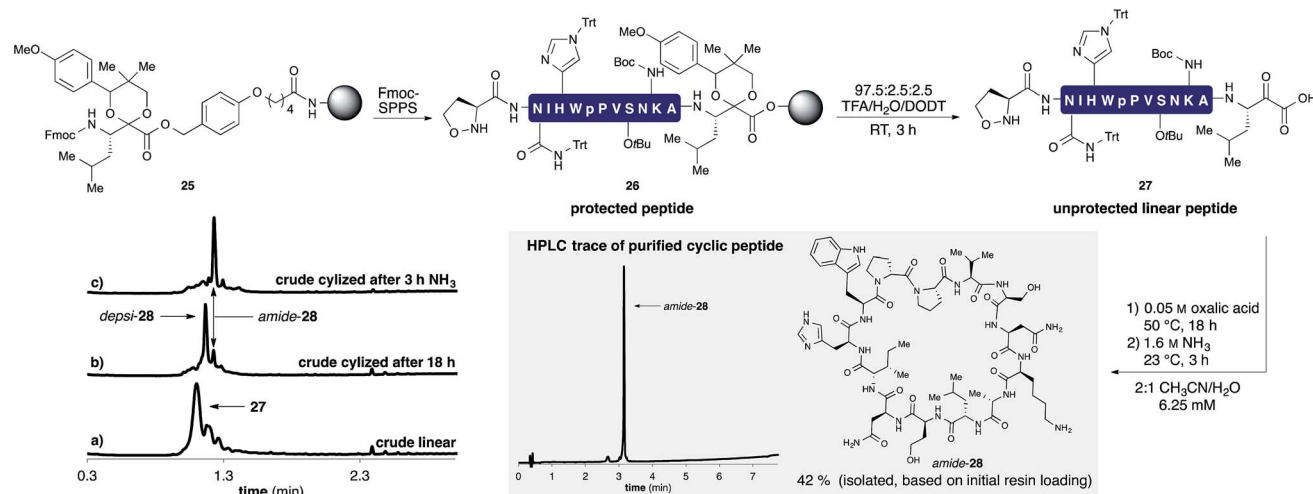
Scheme 5 Synthesis of cyclic peptide amide-28 using the optimized KAH cyclization process. Analytical HPLC traces at 220 nm: (a) crude linear peptide 27 after cleavage from resin. (b) Crude cyclic peptide depsi-28 after 18 h at 50 °C. (c) Crude cyclic peptide amide-28 3 h after the addition of 1.6 M aq NH 3 . [DODT = 3,6-dioxa-1,8-octanedithiol]. 28
