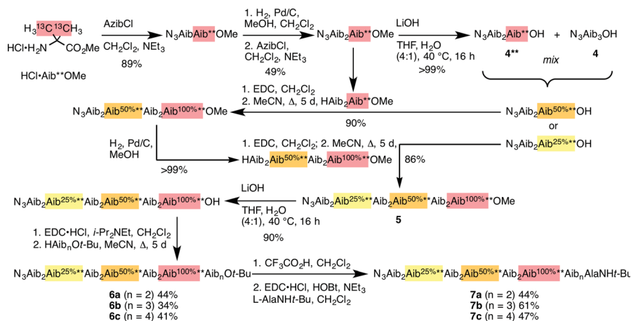
Fig. 5 Synthesis of oligomers 7a–c with residues identified by abundance-labelled ^{13}\text{C} labels.
