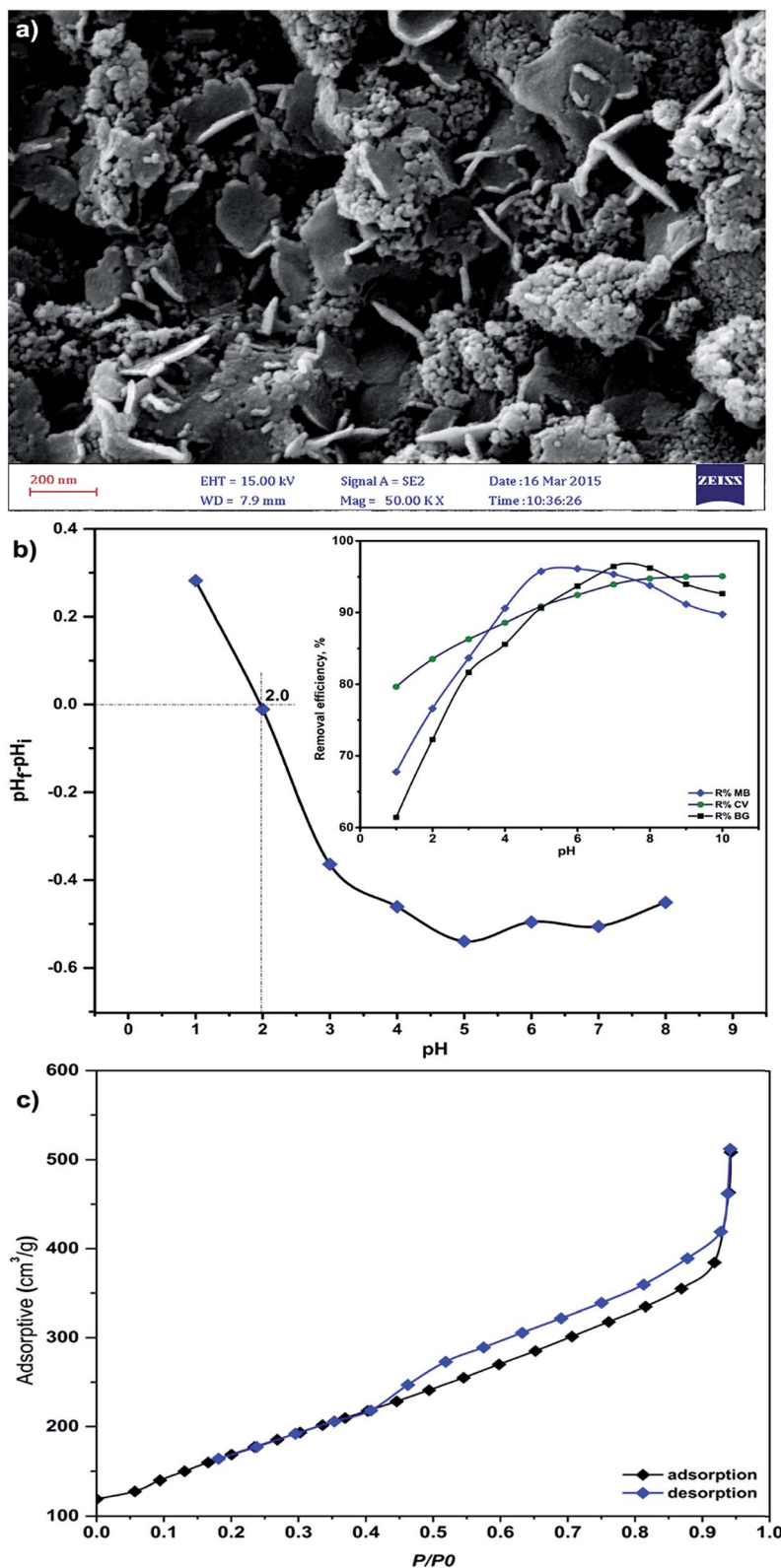
Fig. 4 (a) FESEM image of the prepared \text{MnO}_2\text{-NP-AC} , (b) pHzpc of \text{MnO}_2\text{-NP-AC} ( \text{pH}_i = initial pH and \text{pH}_f = final pH) and (c) nitrogen adsorption–desorption isotherms.
