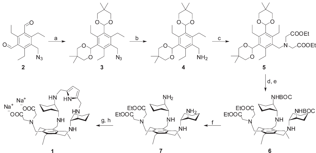
Scheme 1 Synthesis of receptor 1 . Reagents and conditions: (a) neopentylglycol, p-TsOH cat., toluene, reflux, overnight, 87%; (b) LiAlH 4 , THF, r.t., 2.5 h, 92%; (c) ethyl bromoacetate, KHCO 3 , DMF, r.t. overnight, 83%; (d) HCl 1 M, THF, overnight; (e) N -BOC-(1 R , 2 R )-1,2- trans -diaminocyclohexane, CHCl 3 , reflux, overnight, then NaBH 4 suspension in MeOH, r.t., 1 h, 62%; (f) TFA, CH 2 Cl 2 , r.t., 2 h, 79%; (g) pyrrole-2,5-dicarbaldehyde, CHCl 3 , r.t., then NaBH 4 suspension in MeOH, r.t., 1 h, 70%; (h) NaOH, H 2 O/EtOH 1 : 1, r.t., overnight, 81%.
