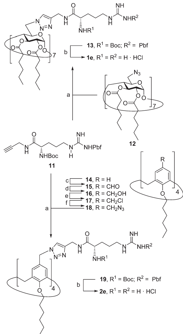
Scheme 3 Synthesis of triazol-linked polyarginine \beta CD and CA_4 "clicked" clusters 1e and 2e . Reagents and conditions: (a) Et_3N , DCM, reflux, 48 h, 99% (for 13 ) or 24 h, 71% (for 19 ); (b) (i) 95 : 2.5 : 2.5 TFA-TIS-H 2 O, rt, 1 h; (ii) 0.1 M HCl, quantitative; (c) (i) hexamethylenetetramine, TFA, reflux, 2 d; (ii) HCl, 3 h, 96%; (d) NaBH_4 , EtOH, 0 °C \rightarrow rt, 18 h, 86%; (e) SOCl_2 , DCM, 4 h, rt, 95%; (f) NaN_3 , DMF, 16 h, 40 °C, 95%.
