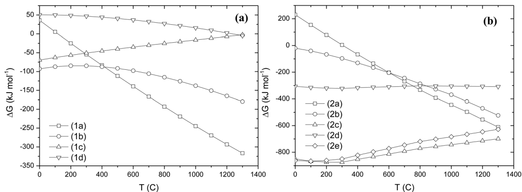
Fig. 8 (a) A plot of the standard Gibbs energy change ( \Delta G^\circ , \text{kJ mol}^{-1} ) per mol of mineral against temperature ( T °C) for: (a) thermal decomposition reactions (1a)–(1d), and (b) alkali roasting reactions (2a)–(2e).
