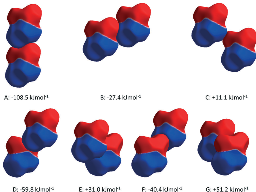
Fig. 4 Contacts A–G in ε-glycine depicted with electrostatic potentials mapped onto Hirshfeld surfaces. The colour scheme spans \pm 0.01 au with positive and negative regions in blue and red, respectively.
