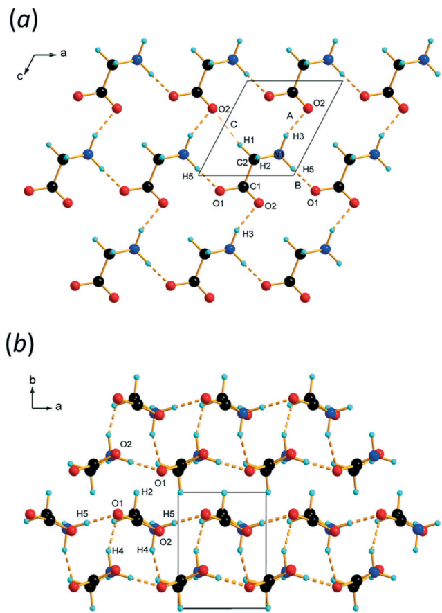
Fig. 3 (a) Layers formed parallel to the ac planes in ε-glycine at 4.3 GPa. (b) Stacking of layers along b .
