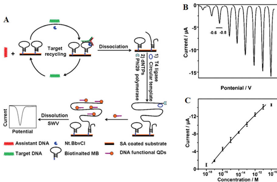
Fig. 6 (A) Schematic illustration of the TEHP amplification strategy for DNA detection, (B) stripping voltammograms of cadmium ions corresponding to (left to right) 10 -18 , 10 -17 , 10 -16 , 10 -15 , 10 -14 , 10 -13 , 10 -12 , 10 -11 , and 10 -10 M of target DNA. (C) The corresponding analytical quantitative dynamic range. Reprinted permission from ref. 46, copyright©2012, American Chemical Society.
