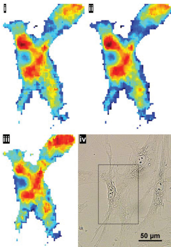
Fig. 8 Example image from a targeted region of cultured human skin fibroblasts measuring \sim 90 \times 50 \mu\text{m} ; Comparing vector normalised, integrated lipid region chemimaps ( 2800\text{--}3000 \text{ cm}^{-1} ) before (i) and after noise reduction (ii) versus the image once the data has been noise-reduced, RMieS-EMSC corrected then vector normalised (iii). The optical image was acquired with a 20 \times objective, at a pixel resolution of 0.53 \mu\text{m} (iv).
