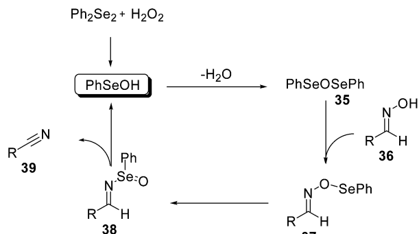
Scheme 29 Aldoximes dehydration.
