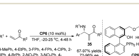
Scheme 17 CP4 or CP5-catalyzed aza-MBH reactions.
