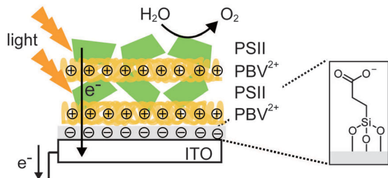
Fig. 9 Layer-by-layer (LbL) assembly of PBV 2+ and PSII on an ITO-coated glass substrate. 33
