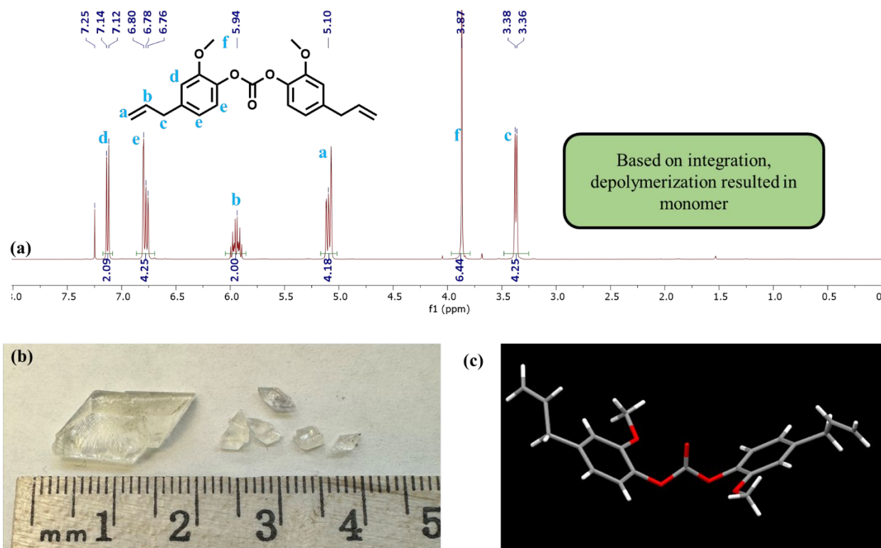
Figure 6. (a) ^1\text{H} NMR spectrum of the ethenolysis product generated from oligomers of the eugenol-based polycarbonates \text{CDCl}_3 . (b) Photograph showing crystalline monomer obtained via ethenolysis. (c) X-ray crystal structure of the monomer. Ortep drawings with thermal ellipsoids at the 50% probability level are included in the supporting information.
