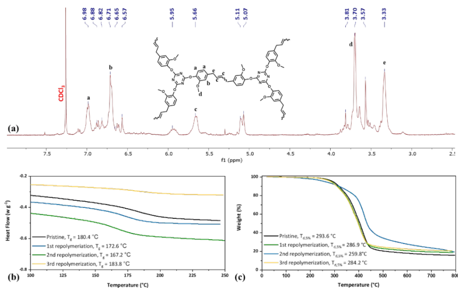
Figure 10. (a) ^1\text{H} NMR of CEN4 and (b) DSC and (c) TGA thermogram of CEN1 – CEN4.
