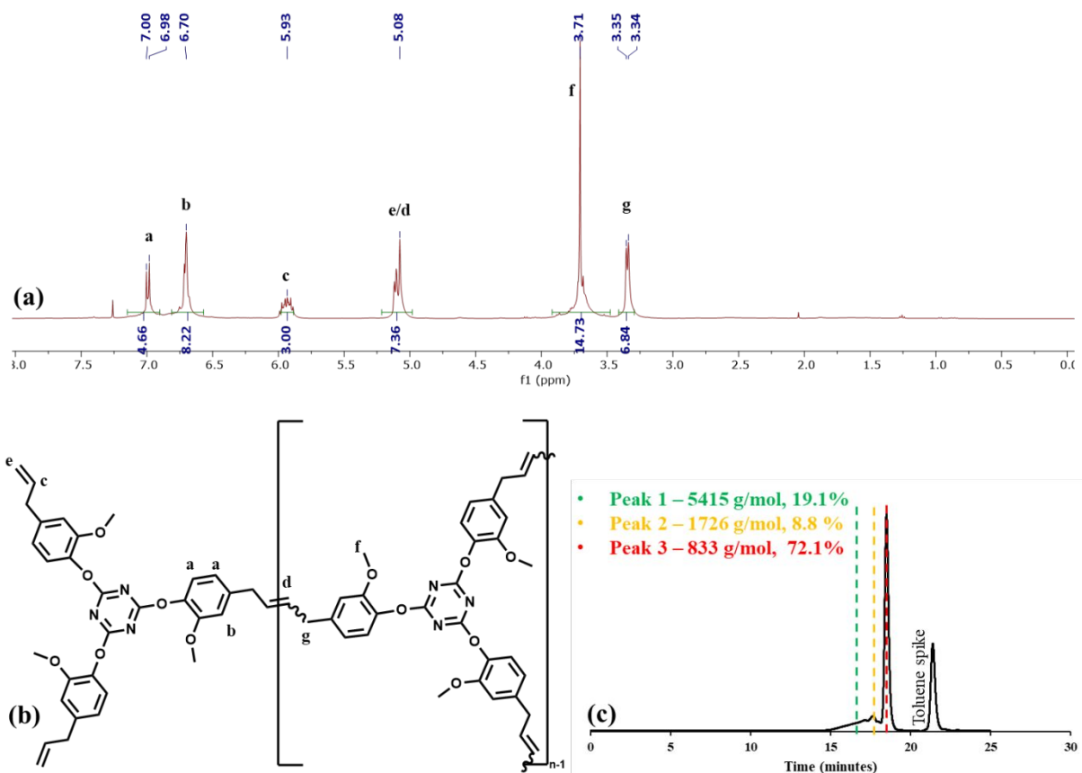
Figure 7. (a) ^1\text{H} NMR spectrum of the CEN1a ethenolysis product in \text{CDCl}_3 . (b) Chemical structure of the ethenolysis product. (c) GPC chromatogram of the ethenolysis product.
