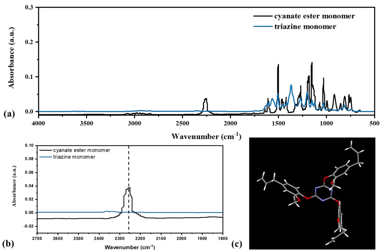
Figure 3. (a) ATR-FTIR spectrum of 3 before and after thermal cyclotrimerization. (b) Expanded view of the -OCN region in the FTIR spectrum. (c) X-ray crystal structure of compound 4 . Ortep drawings with thermal ellipsoids at the 50% probability level are included in the supporting information.
