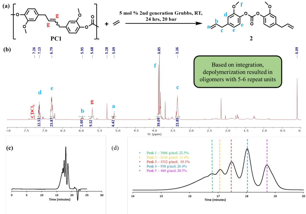
Figure 5. (a) Ethenolysis scheme for depolymerization of polycarbonates. (b) 1 H NMR spectrum of depolymerized PC1 low in CDCl 3 . (c) GPC chromatogram of ethenolysis products derived from PC1 low . (d) Magnified view of the GPC chromatogram of depolymerized PC1 low .
