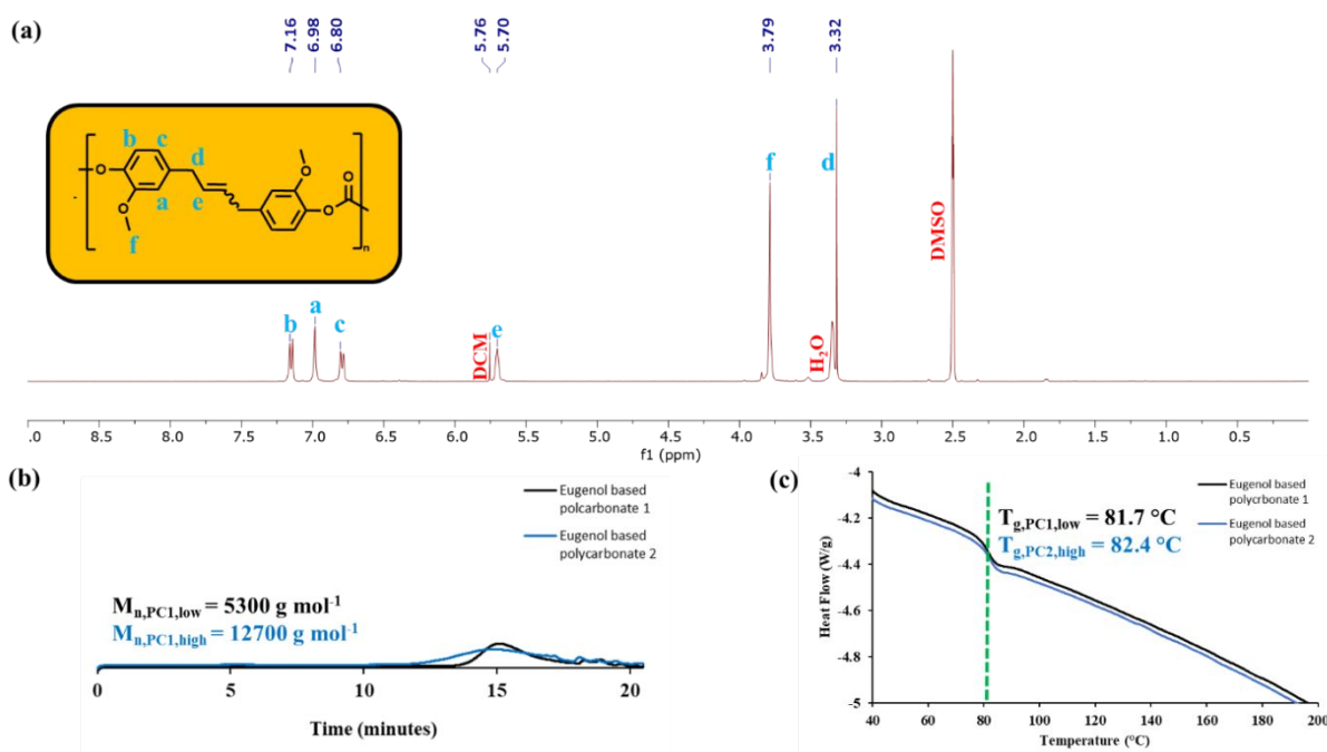
Figure 1. (a) 1 H NMR spectrum of PC1 high in DMSO-d 6 . (b) GPC data for PC1 low and PC1 high . (c) DSC traces for PC1 low and PC1 high . Heating cycles ran from 40 °C – 200 °C at 10 °C/min
