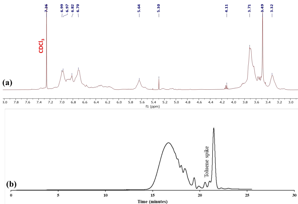
Figure 4. (a) ^1\text{H} NMR spectrum of CEN1 in \text{CDCl}_3 . (b) GPC of CEN1.
