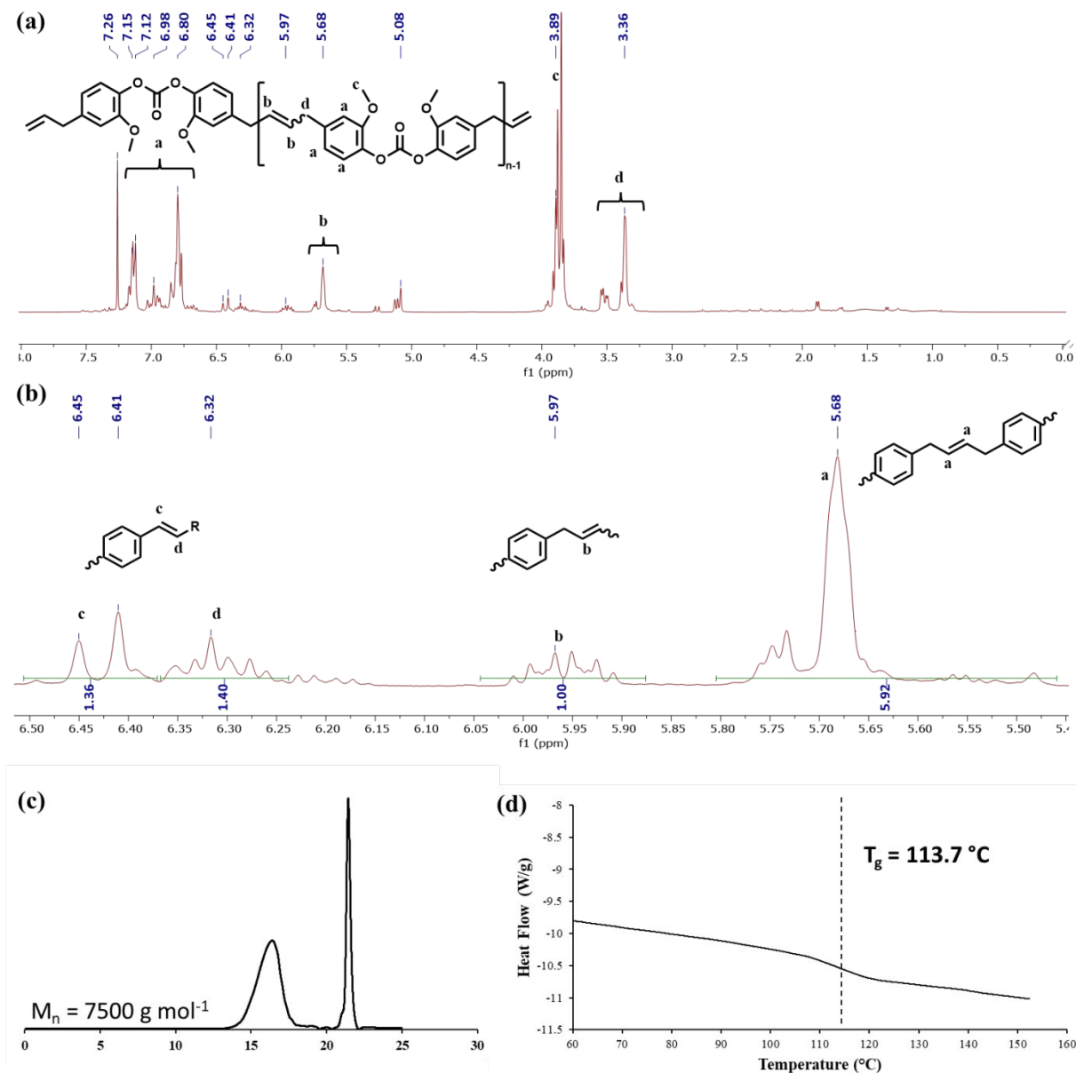
Figure 9. (a) ^1\text{H} NMR spectrum of the repolymerized polycarbonate in \text{CDCl}_3 . (b) Zoomed-in region of ^1\text{H} NMR spectrum showing alkene isomerization. (c) GPC chromatogram of the repolymerized polycarbonate. (d) DSC thermogram of the repolymerized polycarbonate.
