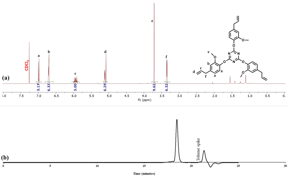
Figure 8. (a) 1 H NMR spectrum of fully depolymerized polycyanurate (CEN1b) in CDCl 3 . (b) GPC chromatogram of CEN1b
