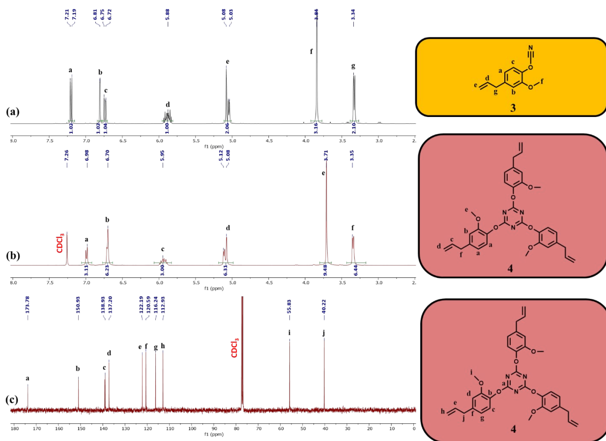
Figure 2. (a) ^1\text{H} NMR spectrum of 4-allyl-1-cyano-2-methoxybenzene (compound 3 ) in \text{CDCl}_3 . (b) ^1\text{H} NMR spectrum of 2,4,6-tris(4-allyl-2-methoxyphenoxy)-1,3,5-triazine (compound 4 ) in \text{CDCl}_3 generated via thermal cyclotrimerization of 3 . (c) ^{13}\text{C} NMR of compound 4 in \text{CDCl}_3 .
