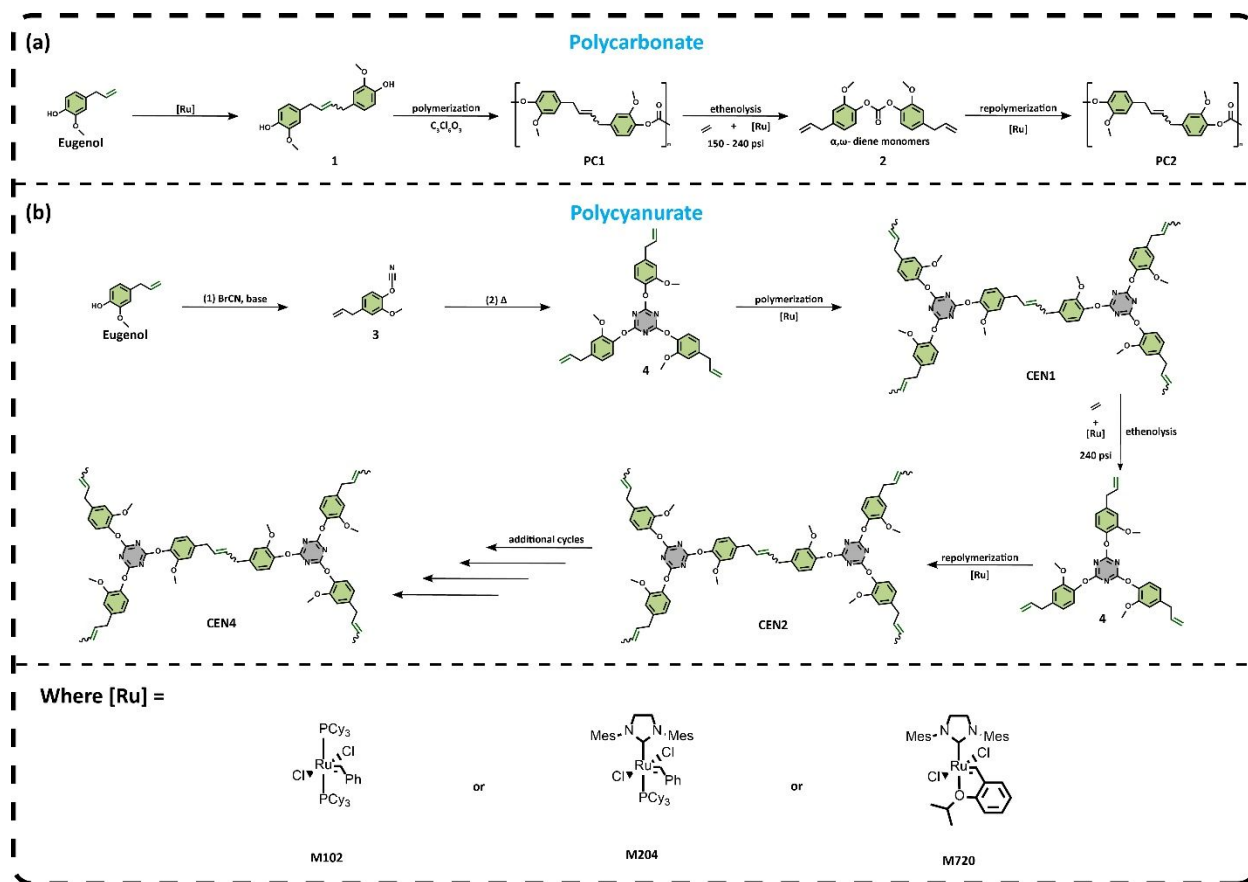
Scheme 1. (a) Bisphenol synthesis, polymerization, ethenolysis, and repolymerization of eugenol-based polycarbonates. (b) Cyanation, thermal trimerization, network synthesis, ethenolysis, and subsequent rounds of repolymerization and ethenolysis.
