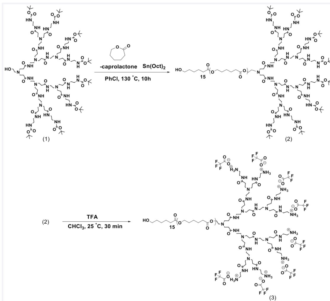
Scheme 1. General synthetic route to LDBC by ring-opening polymerization of \epsilon -caprolactone monomer initiated by PAMAM-G3-Boc macroinitiator. 11
