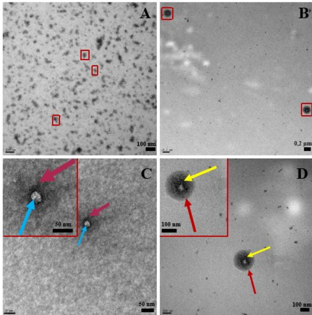
Figure 4. Room temperature TEM of LDBC (A and C) and IL-LDBC nanoparticles (B and D) show different morphologies. C and D show zoomed-in regions of nanoparticles shown in A and B, respectively. In C, the LDBC
