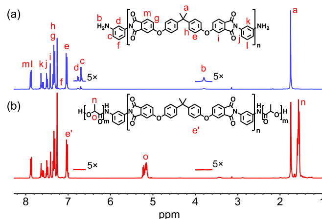
Fig. 2 Representative 1 H NMR spectra of (a) PEI-45 and (b) AIA-45. According to the integrated areas of peak o and e', the weight fraction of PLA in AIA was 38.8%.
