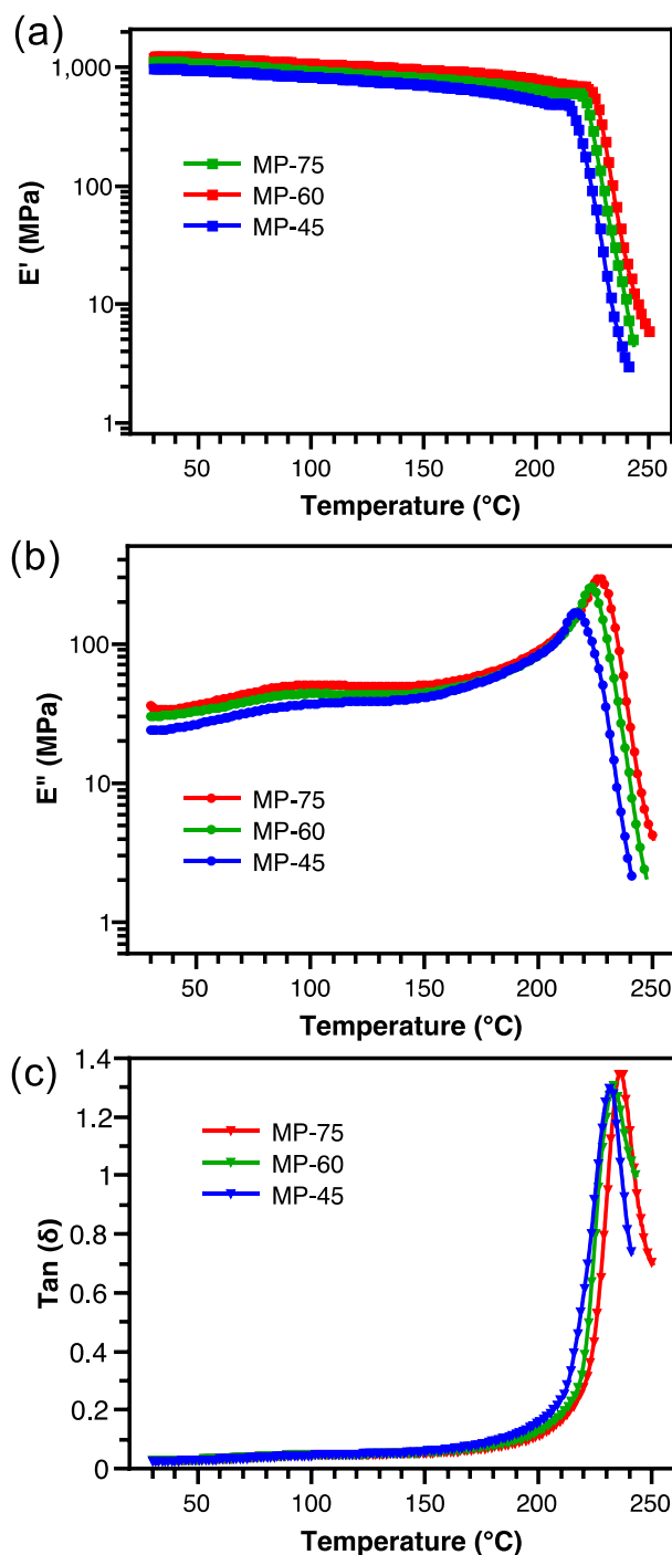
Fig. 7 Dynamic mechanical analysis of mesoporous PEI films after hydrolysis: (a) storage moduli, (b) loss moduli and (c) \text{tan}(\delta) of MP-45, -60 and -75.
