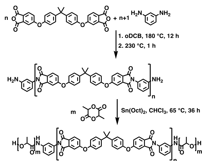
Scheme 1 Synthesis of AIA. PEI-NH 2 was synthesized via condensation polymerization of BPADA and mPD. The amine end groups in PEI initiated ring-opening polymerization of PLA to produce AIA triblock copolymers.
