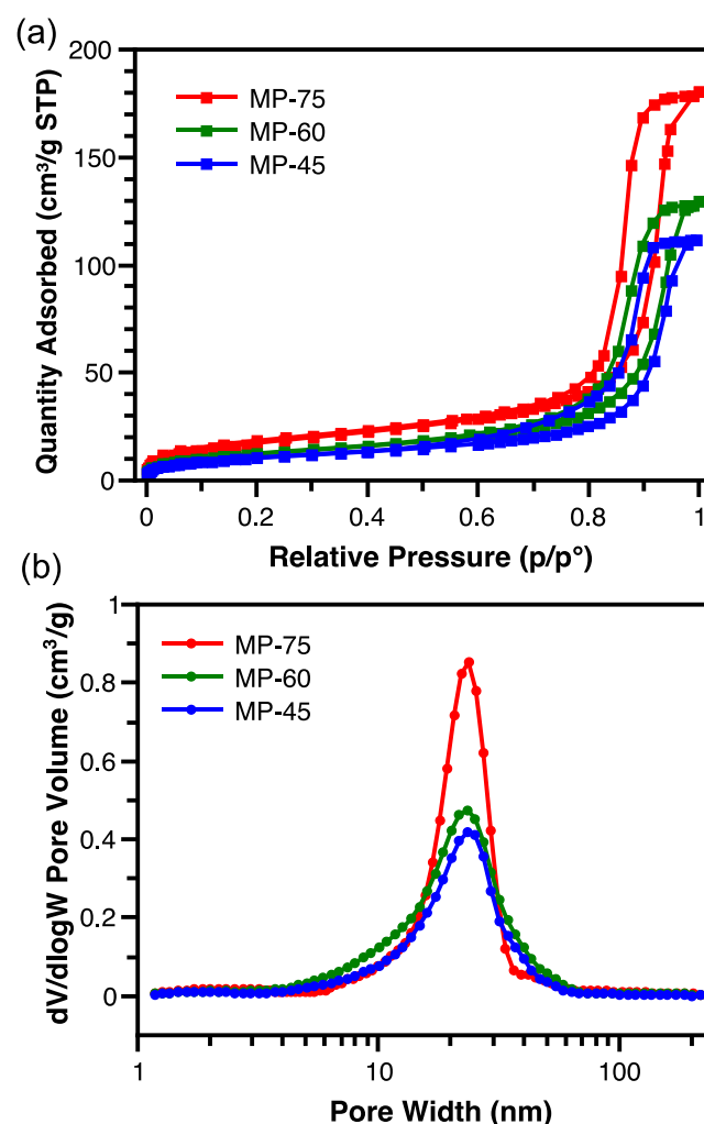
Fig. 5 Nitrogen sorption isotherms and pore size distributions of mesoporous PEI films. (a) The isotherms show specific surface areas of 36, 42 and 61 m 2 /g for MP-45, -60 and -75, respectively. (b) The pore size distributions display an average pore width of 24 nm for all MP films.
