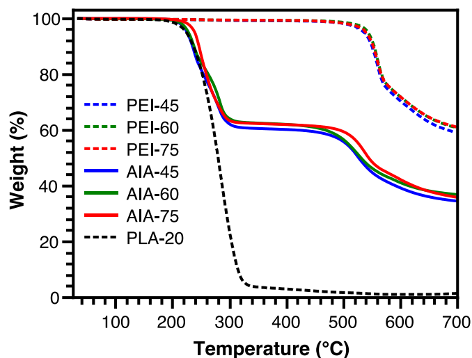
Fig. 3 TGA of AIA, PEI and PLA. The first and second weight loss of AIA at 180 – 300 °C and above 450 °C corresponded to the thermal decomposition of PLA and PEI, respectively. According to the weight loss, the weight fractions of PLA in AIA-45, -60 and -75 were 39.8%, 38.1% and 38.0%, respectively.
