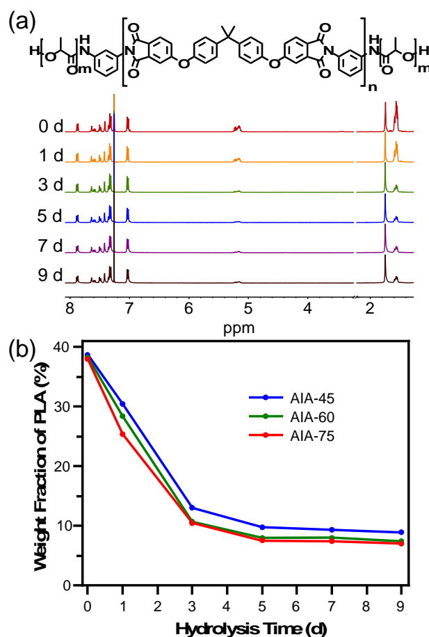
Fig. 6 Hydrolysis rate of AIA films in phosphate buffer solution. (a) ^1\text{H} NMR spectra display a decreasing signal of PLA repeating units in AIA-45. (b) The PLA weight fractions in all AIA films were below 9% after hydrolysis for 9 days.
