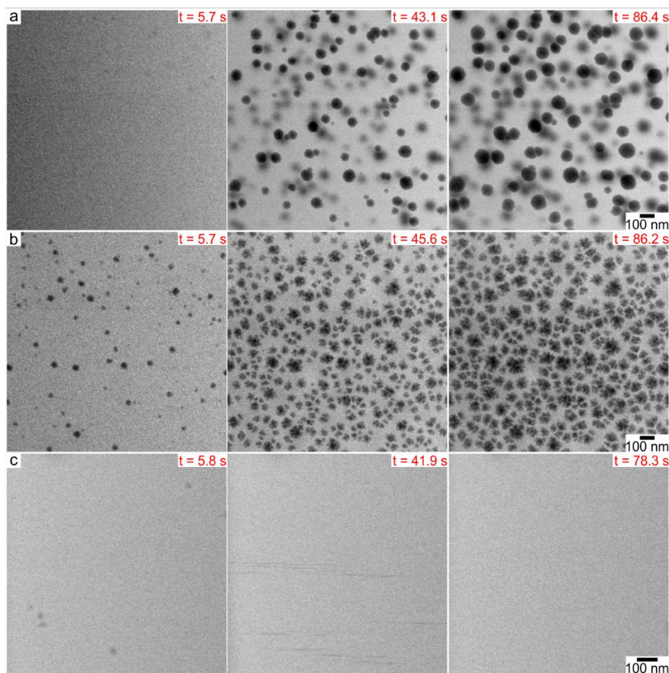
Figure 1. Time lapsed LP-TEM images of Pt nanoparticle formation demonstrate precursor chemistry affects particle morphology and growth dynamics. (a) Spherical and faceted nanoparticle growth in the presence of 1 M TBA (beam current of 31 pA, magnification of 120 kx, and dose rate of 1.9 MGy/s). (b) Dendritic nanoparticle growth in DI water (beam current of 31 pA, magnification of 120 kx, and dose rate of 1.9 MGy/s). (c) Spherical nanoparticle growth followed by nanoparticle detachment in the presence of 1 M TBA and 1 mM SC (beam current of 107 pA, magnification of 200 kx, and dose rate of 17.9 MGy/s).
