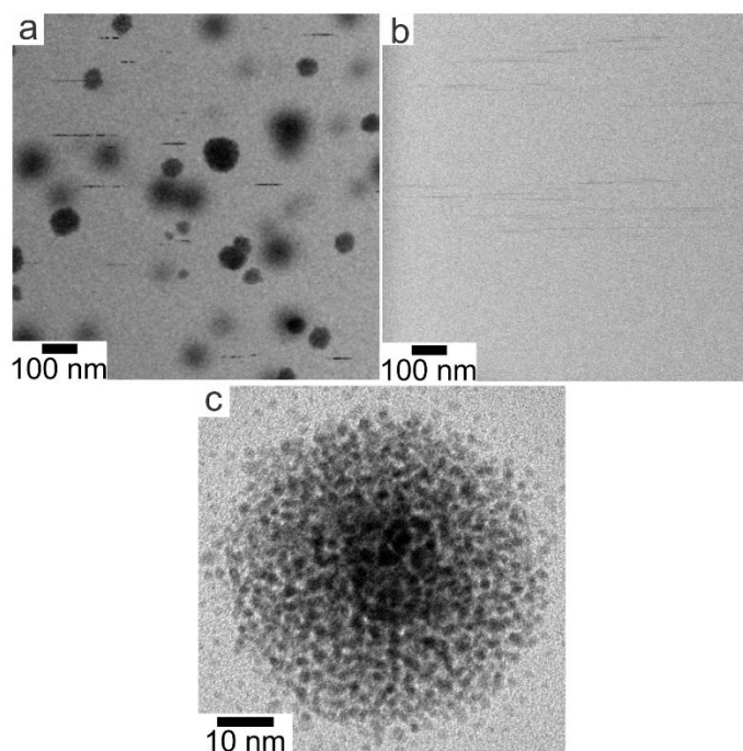
Figure 3. LPTEM and dry HRTEM images indicate supraparticles formed by assembly of 2 nm primary particles formed in bulk solution. (a)-(b) Bright field LP-TEM images showing horizontal steaks in (a) 1 M TBA (pixel dwell time of 25 \mu s and frame rate of 0.04 frames/s) and (b) 1 M TBA and 1 mM SC (pixel dwell time of 5 \mu s and frame rate of 0.2 frames/s). (c) Dry state HRTEM image showing free platinum primary particles attached to the substrate near a supraparticle.
