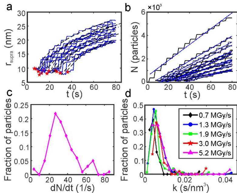
Figure 4. Supraparticle assembly kinetics were diffusion limited. (a) Platinum supraparticle radius as a function of time (solid blue lines) and non-linear least squares fits of equation (1) (black dashed lines). Experimental nucleation times are shown as red stars. (b) Estimated number of platinum primary nanocrystals in each supraparticle as a function of time. Blue dashed lines are linear least squares best fits of equation (2). (c) Histogram of the primary nanoparticle attachment rate distribution. The experimental conditions for the growth rate data in (a)-(c): beam current of 31 pA, magnification of 100 kx, and dose rate of 1.3 MGy/s. (d) Distribution of growth coefficients, k , of platinum supraparticles at different dose rates.
