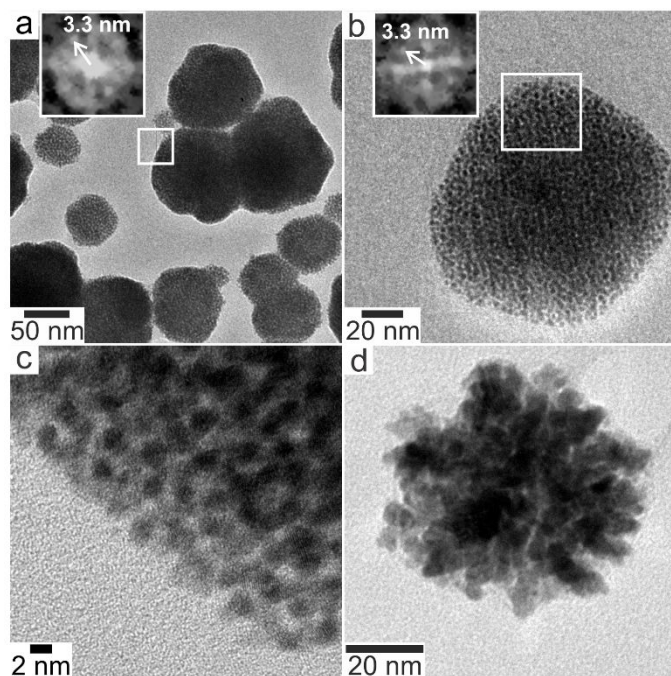
Figure 2. Dry-state HRTEM images after LPTM experiments showed Pt supraparticles were comprised of close-packed primary particles displaying amorphous and crystalline domains. (a-c) Supraparticles synthesized in the presence of 1 M TBA precursor. (d) Supraparticle synthesized in DI water. The white boxes in (a) and (b) indicate where the inset FFTs were taken.
