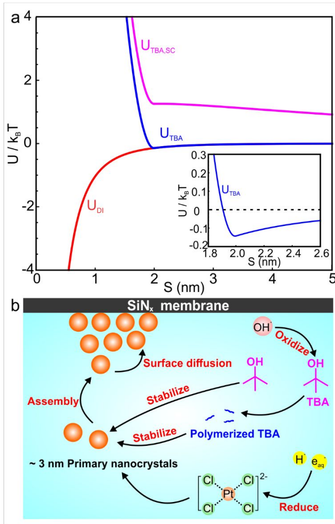
Figure 5. Interparticle interaction model demonstrates sub- k_B T attractive potentials underlying primary particle assembly in the presence of TBA and enable rapid surface diffusion of primary particles. (a) The pairwise interaction potential energy as a function of surface-to-surface separation ( S ) between two 3 nm diameter platinum nanocrystals in solution. U_{DI} (red curve) corresponds to DI water only, U_{TBA} corresponds to TBA in DI water, and U_{TBA,SC} (magenta curve) corresponds to TBA and SC in DI water. (b) Schematic showing the overall proposed mechanism for platinum nanoparticle formation in the presence of TBA.
