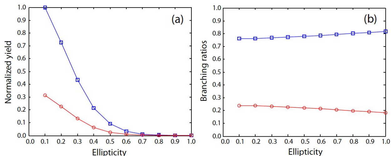
Figure 3: (a) Calculated ionization rates for two fictitious atoms with ionization potentials of 32 eV (blue) and 33 eV (red) with varying ellipticities. (b) The computed branching ratios using data from Fig. 3a.
