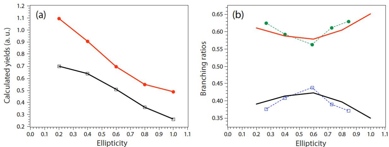
Figure 5: (a) The computed yield variation with laser ellipticity for sequential double ionization via a \pi cation (red) and a \sigma cation (black). (b) The branching ratio variations of the \pi cation ionization (red) and the \sigma cation ionization (black) calculated using data from Fig. 5a., showing a minimum/maximum peak at \epsilon=0.6 . For comparison, the experimental branching ratios of \text{CH}_3^+ dissociation channel (blue square) and the sum of the other three channels (green dot), are also shown for ellipticity between 0.27 and 0.85. Data for lower ellipticity at 0.05 and 0.11 were not shown because they are dominated by NSDI.
