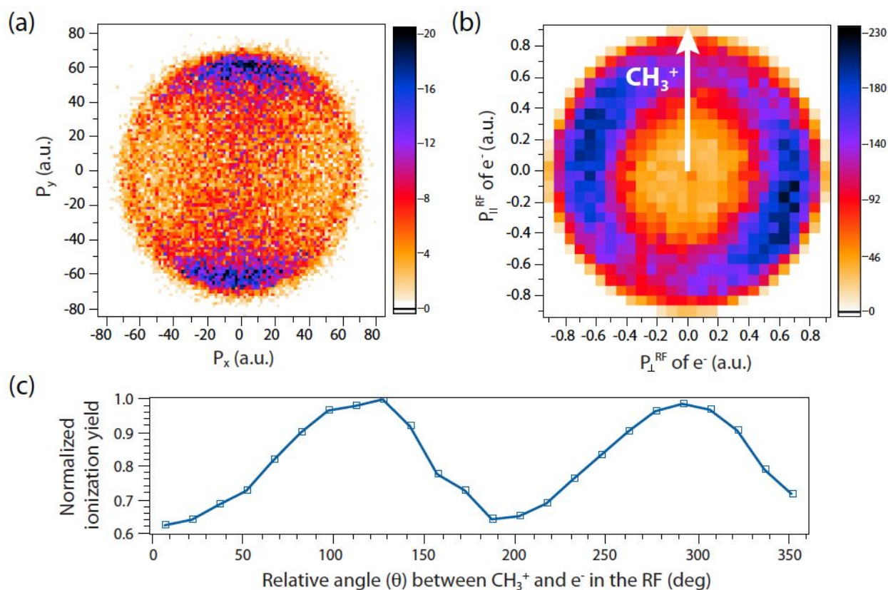
Figure 6: (a) The (x,y) momentum distribution of \text{CH}_3^+ dissociation in the plane perpendicular to the laser polarization plane ( y, z ). (b) The RF-PAD of electrons in coincidence with \text{CH}_3^+ dissociation. The plot was obtained by having the \text{CH}_3^+ momentum vector pointing up in the figure while rotating the coincident electron momentum vector accordingly. All momentum vectors are in the plane of polarization ( y, z ). The helicity of the laser was clockwise. (c) Integrated 1D RF-PAD.
