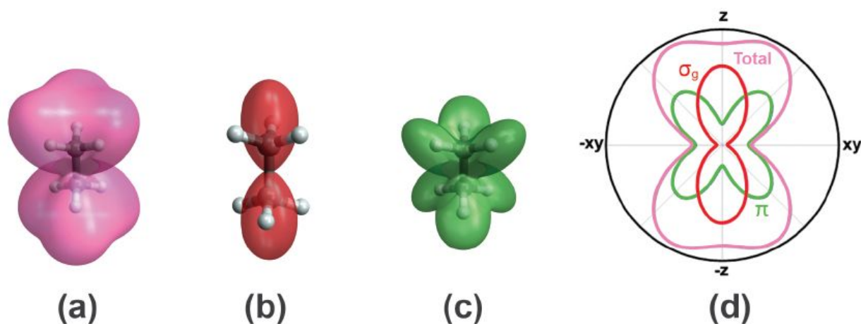
Figure 4: (a) Calculated total ionization yield of neutral ethane. (b) and (c) The breakdown of the total yield to the MO contributions from \sigma_g and the doubly degenerate \pi_g/\pi_u orbitals, respectively. (d) Total angular dependence of ionization yield (pink) with respect to the polar angle about the C-C bond (z-axis). For each polar angle, the ionization yield has been averaged over the azimuthal directions in the xy plane; and the corresponding ionization contributions from the \pi_g/\pi_u orbitals (green) and \sigma orbitals (red).
