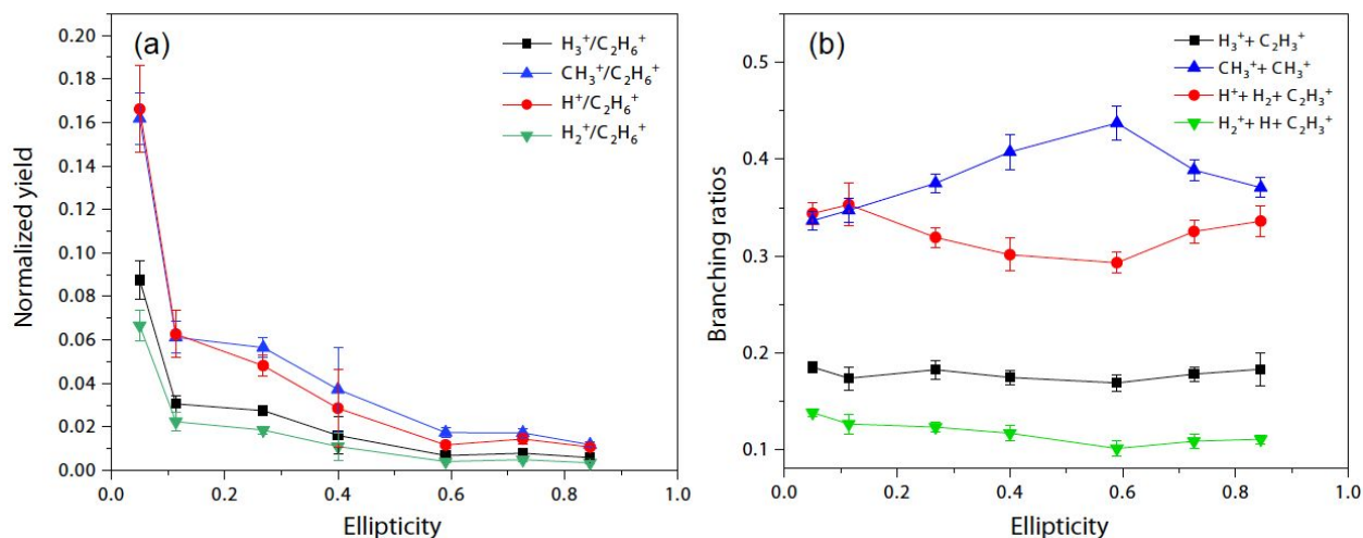
Figure 2: (a) Normalized yields of different dissociation channels. (b) Ellipticity dependent branching ratios of different dissociation channels.
