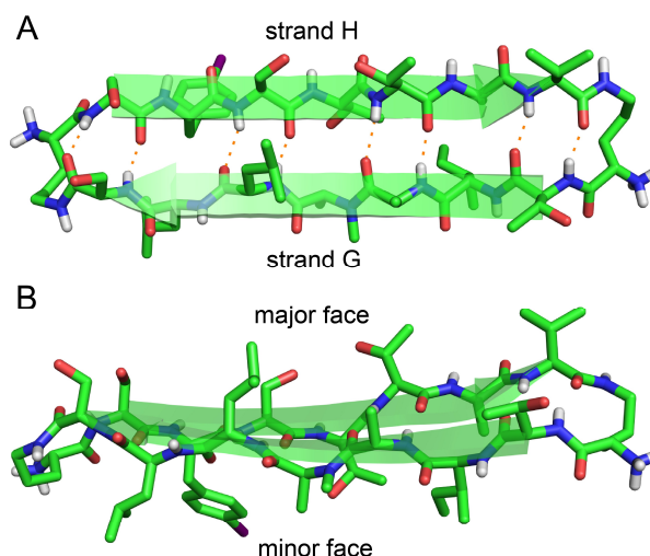
Figure 3. X-ray crystallographic structure of peptide 1 (PDB 5HPP). (A) Hydrogen-bonded \beta -hairpin monomer. (B) Side view of the \beta -hairpin monomer.
