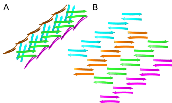
Figure 6. (A) Square channel. (B) Square channel unrolled and flattened.
