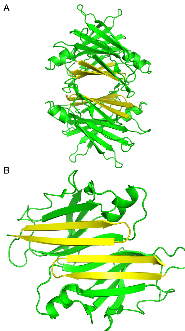
Figure 1. (A) X-ray crystallographic structure of the TTR tetramer. The \beta -hairpin of the tetramer interface is highlighted in yellow (PDB 1DVQ). 18 (B) TTR dimer subunit.
