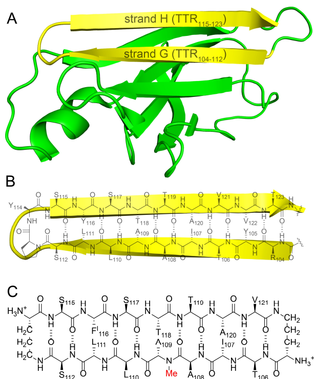
Figure 2. (A) TTR monomer. The \beta -hairpin comprising \beta -strands G and H is highlighted in yellow. (B) Cartoon and chemical structure of the \beta -hairpin comprising \beta -strands G and H. (C) Chemical structure of peptide 1.
