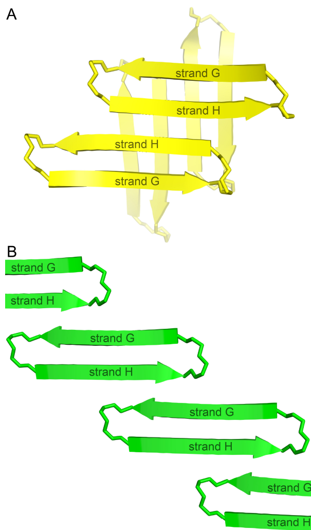
Figure 8. (A) Hypothesized tetramer of peptide 1 . (B) Crystallographically observed extended \beta -sheet formed by peptide 1 .
