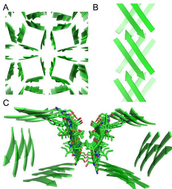
Figure 7. (A) Tilted windows assembly of square channels. (B) Side view of the interface between two square channels. (C) Hydrophobic contact between two square channels.
