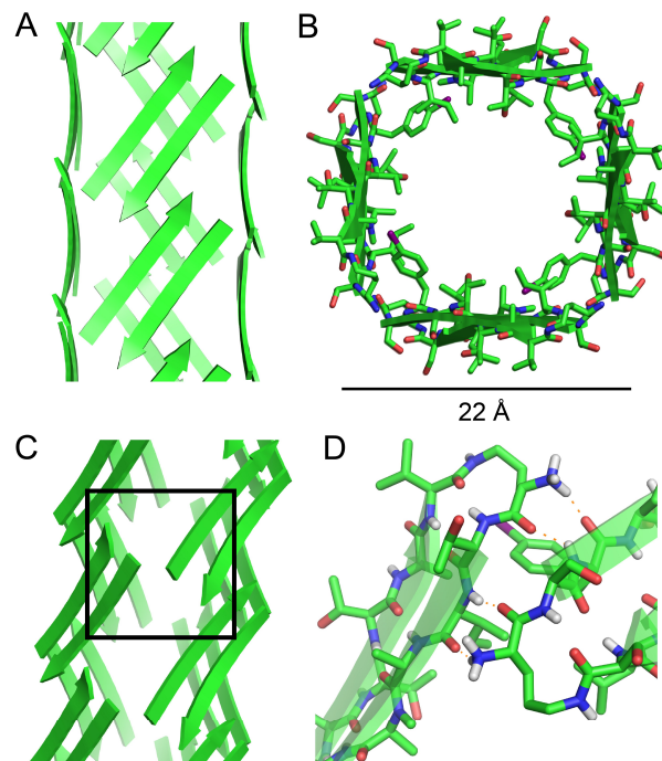
Figure 5. Square channel formed by peptide 1. (A) Side view. (B) Top view. (C) Corner view. (D) Detail showing hydrogen-bonding interactions between \beta -sheets at the corner of the square channel.
