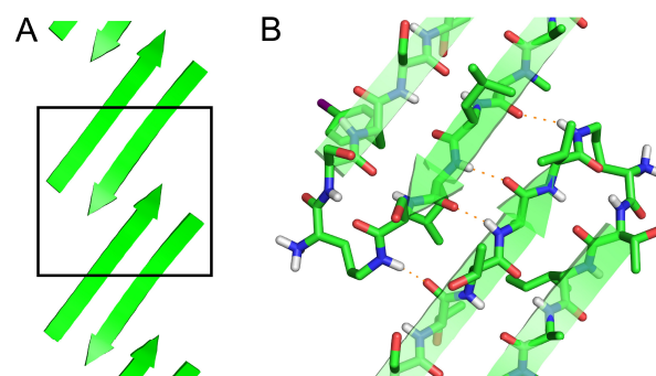
Figure 4. (A) Extended \beta -sheet formed by peptide 1. (B) Detail showing hydrogen-bonding interactions between \beta -sheets.
