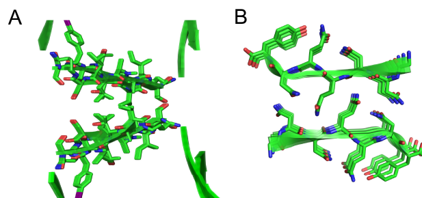
Figure 10. (A) Interface between square channels in the tilted windows assembly. (B) Steric zipper formed by a peptide from the yeast prion protein Sup35 (PDB 1YJP).
