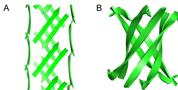
Figure 9. (A) Square channel formed by peptide 1 . (B) Cylindrin formed by a peptide fragment from \alpha B crystallin (PDB 3SGO).
