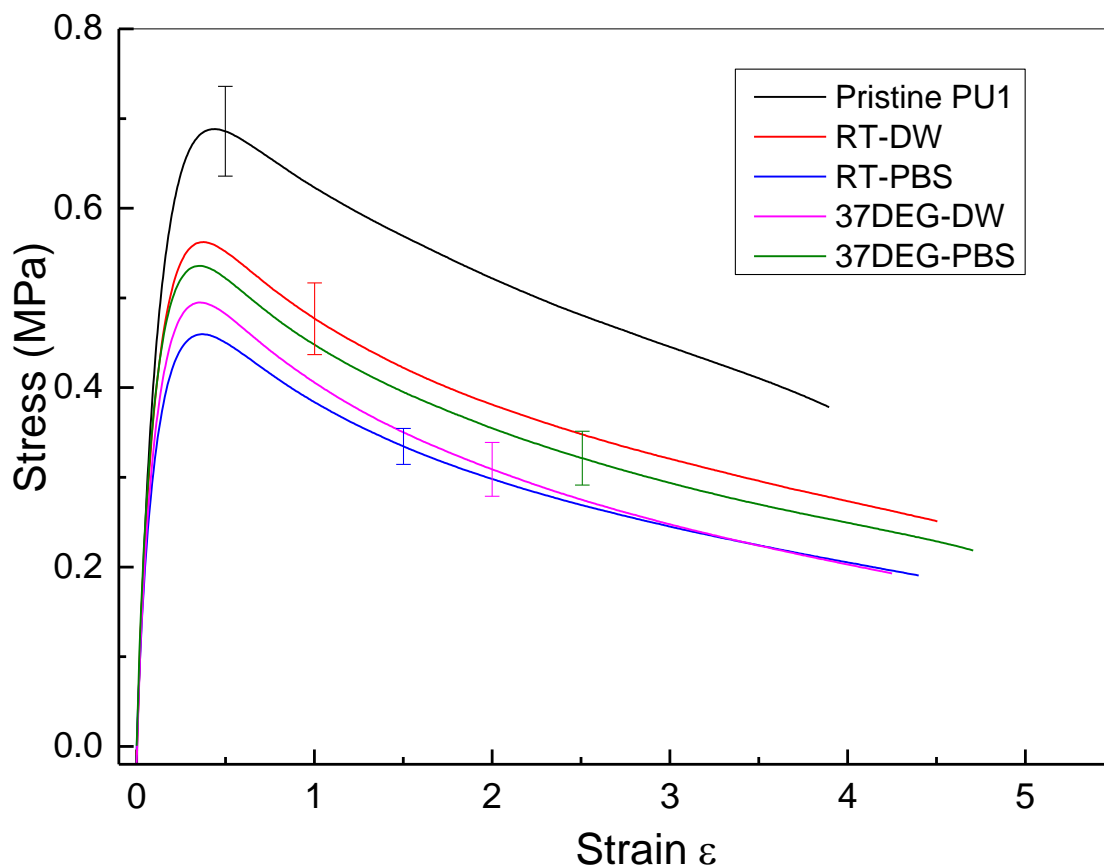
Fig. 6 Mean stress-strain curve for pristine and polyurethane 1 at different physiological conditions. Pristine PU1) pristine polyurethane 1 , RT-DW) at room temperature in distilled water for 48 hours, RT-PBS) at room temperature in PBS solution for 48 hours, 37 DEG-DW) at 37 °C in distilled water for 12 hours and 37 DEG-PBS) at 37 °C in PBS solution for 12 hours. Samples were wiped dry before testing.
