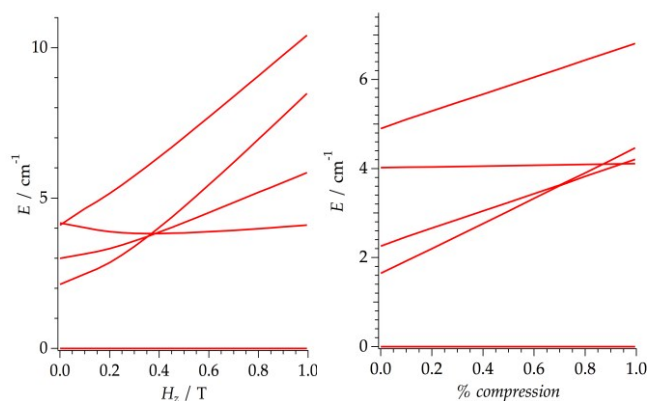
Figure 4: Evolution of the five lowest energy levels of HoPd12 versus (left) magnetic field between 0 and 1 T at an axial compression of 0.8 % and (right) % of axial compression between 0 and 1% at a magnetic field of 0.41 T.
