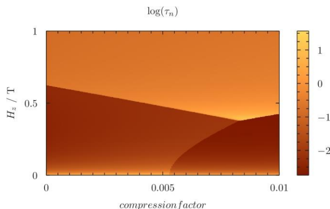
Figure 3: Variation of the decoherence time in logarithmic scale, \log(\tau_n) , considering the coupling to the nuclear spin bath. Vertical axis: applied magnetic field, in Tesla. Horizontal axis: axial compression factor ( \Delta z/z ) of the equilibrium distance.
