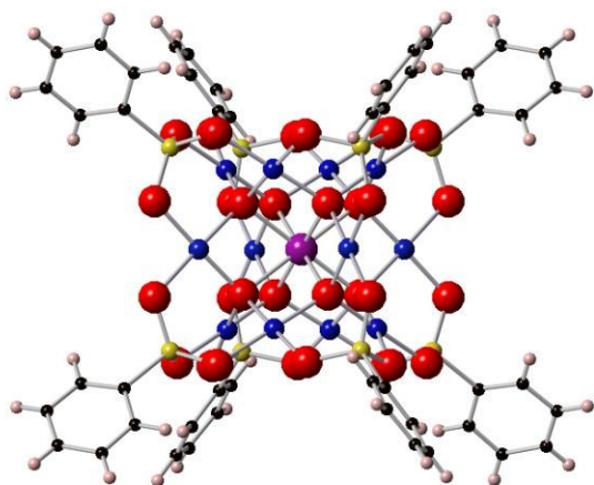
Figure 1: Ball and stick representation of LnPd12. Color code: Ln (violet), O (red), Pd (blue), C (black), As (yellow) and H (pink).
