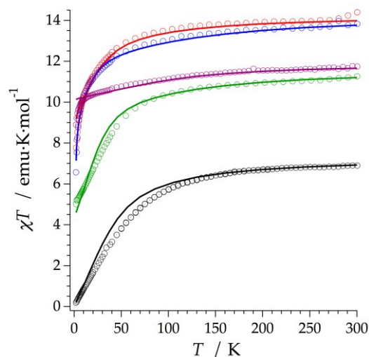
Figure 2: Fitting of the experimental \chi T product of the series of LnPd12 using the REC model: Dy (red), Ho (blue), Tb (violet), Er (green), Tm (black). Open circles stand for experimental data and solid lines represent theoretical fit for structures 1-4 and prediction for 5 .
