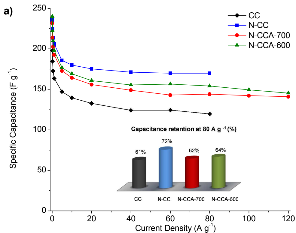
Figure 7. (a) Variation of specific capacitance with increasing discharge current density for the N-doped carbon capsules N-CC, N-CCA-700, N-CCA-600 and the undoped carbon capsules (CC) at 1.1 V in 1 M \text{H}_2\text{SO}_4 . Inset: percentage of capacitance retention at 80 \text{ A g}^{-1} .
