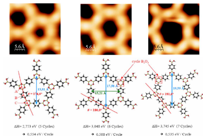
Fig. 6. STM images of closed polygonal pores (pentagons to heptagons, up) and corresponding models from DFT calculations (bottom). The calculated enthalpies of formation per boroxine cycle are reported and vary only within \pm 10\% between the different pore shapes. Adapted from Ref. 41 and Ref. 15 , copyright (2011) American Physical Society.
