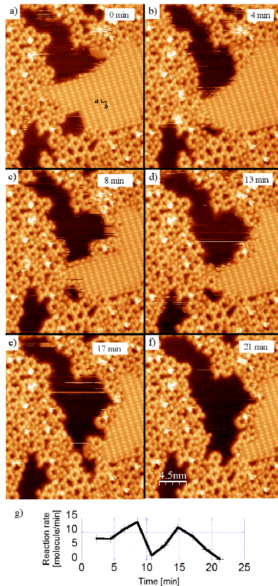
Fig. 4. Sequential STM images ( 28 \times 28 \text{ nm}^2 ) showing the advancement of the polymerisation reaction of BDBA on Ag(100) from the hydrogen bonded phase (a – f). Stable domain boundaries are those along b (long intermolecular distance) or a (short intermolecular distance), or those in direct contact with oligomers. These images were obtained with similar experimental protocol as described in Ref. 42 . g) Evolution of the reaction rate calculated from the disappearance of the molecules in the H-bonded phase.
