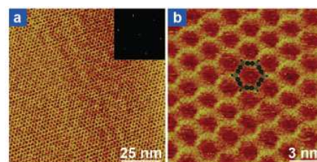
Fig. 11. STM images of the perfect honeycomb network grown from biphenyl-diboronic acid in chemical equilibrium conditions (annealed in the presence of water pressure). Adapted from Ref. 78 .
