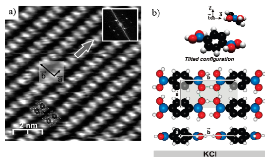
Fig. 2. Deposition of BDBA on KCl(001), a weakly interacting substrate, leads to the formation of a dense hydrogen-bonded phase. a) nc-AFM image. b) Corresponding model of the unit cell showing the tilted configuration of the benzene ring.
