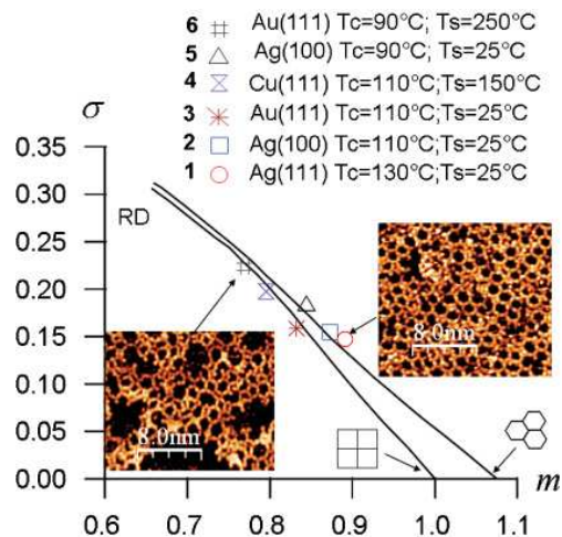
Fig. 7. (m, \sigma) diagram of the minimal spanning tree (MST) statistical analyses for different BDBA polymer networks. T_c refers to the deposition flux (90°C=low flux, 110°C=high flux) and T_s refers to the substrate temperature during deposition. Adapted from Ref. 15 , copyright (2011) American Physical Society.
