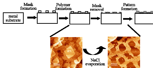
Fig. 10. Schematics of the sequential strategy taking use of self-assembly processes and of the high thermal resistance of boronic acid based 2D polymer in a lithography-mimicking sequence. On a Ag(100) surface, the mask is constituted by square-shaped NaCl islands and the polymer is formed from BDBA precursors. Bottom: STM images of BDBA polymer surrounding NaCl islands (left) and of the square-patterned BDBA polymer after annealing and NaCl evaporation (right). Adapted with permission from Ref. 72 , copyright (2012) Wiley-VCH Verlag GmbH & Co. KGaA, Weinheim.
