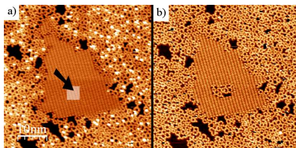
Fig. 5. Local initiation of BDBA polymerisation reaction by manipulation with the STM tip. Inside a hydrogen-bonded domain (indicated by the arrow in (a)) the tip-surface distance was reduced to remove some of the molecules. This resulted in immediate reaction in the modified area (b). Adapted from Ref. 42 .
