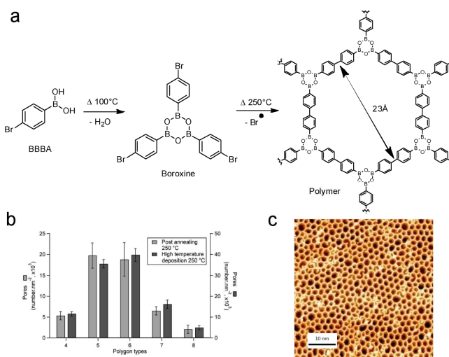
Fig. 9. (a) Reaction scheme for the sequential polymerisation of 1-bromobenzene-4-boronic acid (BBBA) through boronic acid self-dehydration followed by Ullmann radical coupling. (b) Distribution of the polygonal pore shape for room temperature post-annealed and hot substrate depositions. (c) STM image of the high quality 2D polymer obtained by hot substrate deposition. Adapted with permission from Ref. 68 . Copyright (2012) American Chemical Society.
