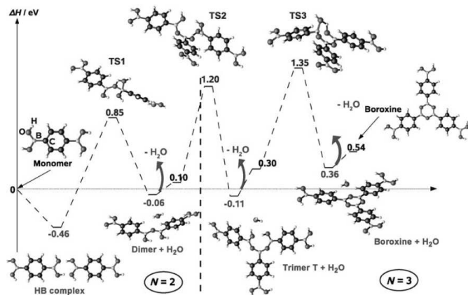
Fig. 3. Boroxine formation reaction mechanism as calculated by DFT. The first step is the formation of a hydrogen-bonded dimer, which represents the only exothermic step. In each transition step, boron becomes tetravalent and relaxes by releasing a water molecule. Reprinted with permission from Ref. 44 , copyright (2009) Wiley-VCH Verlag GmbH & Co. KGaA, Weinheim.
