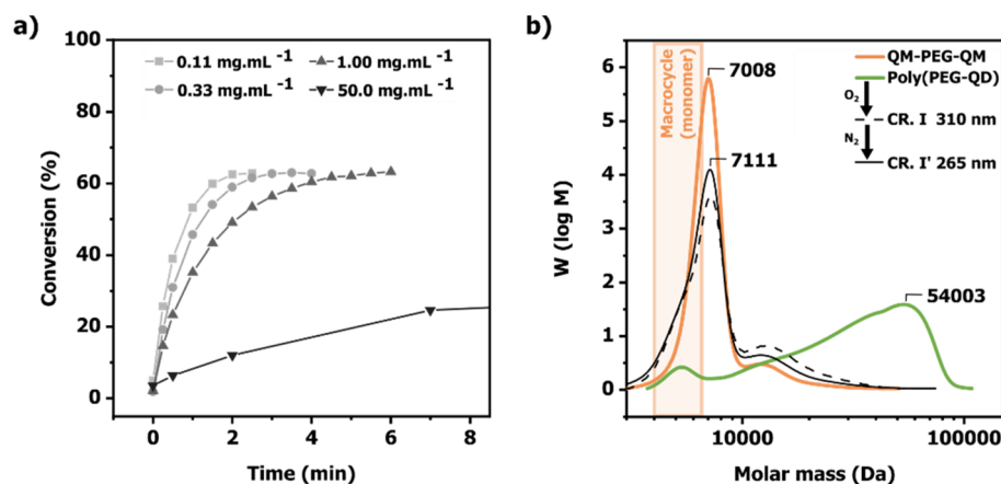
Fig. 5 (a) Comparison of the conversions over time of the cycloreversion of poly(PEG-QD) into QM-PEG-QM through irradiation at 310 nm under oxygenated conditions for different concentrations (from 0.11 to 50 \text{mg mL}^{-1} ) of poly(PEG-QD) . (b) Comparison of the GPC chromatograms of QM-PEG-QM (orange line), poly(PEG-QD) (green line), the cycloreversion (CR.I) of poly(PEG-QD) through irradiation at 310 nm under oxygenated conditions at c = 0.33 \text{ mg mL}^{-1} (black dashed line), and the follow-up irradiation (CR.II) at 265 nm under oxygen-free conditions, at c = 0.33 \text{ mg mL}^{-1} (black solid line). The photoreactions were carried out in ACN solutions using an LED photoreactor at power levels ranging from 60 to 80 mW.
