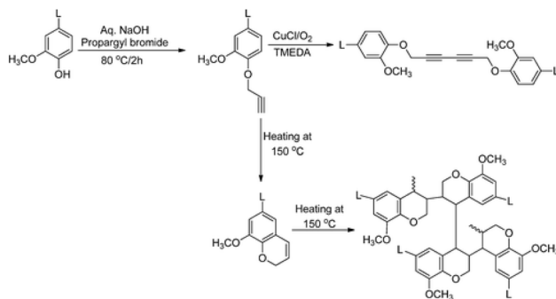
Fig. 17 Lignin chain elongation strategies. The lower part of this schematic displays the Claisen rearrangement and the ensuing thermal polymerization referred to in the text. Reproduced from ref. 179 with permission from the American Chemical Society, copyright 2013.
