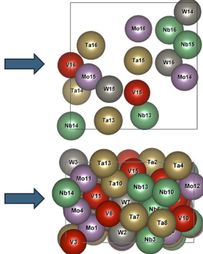
Fig. 2 Bird's eye view of surface atoms (top) and side view (bottom) of (100)-NbTaMoW and (100)-NbTaMoWV slabs. An NPT simulation was conducted on both (100)-RHEA slabs for 100 ps at 800 K to equilibrate the slab volume and atomic configuration at the given temperature. Only the surface atoms are depicted in the bird's eye view (top) with the atoms in the bottom layers filtered out from the image.
