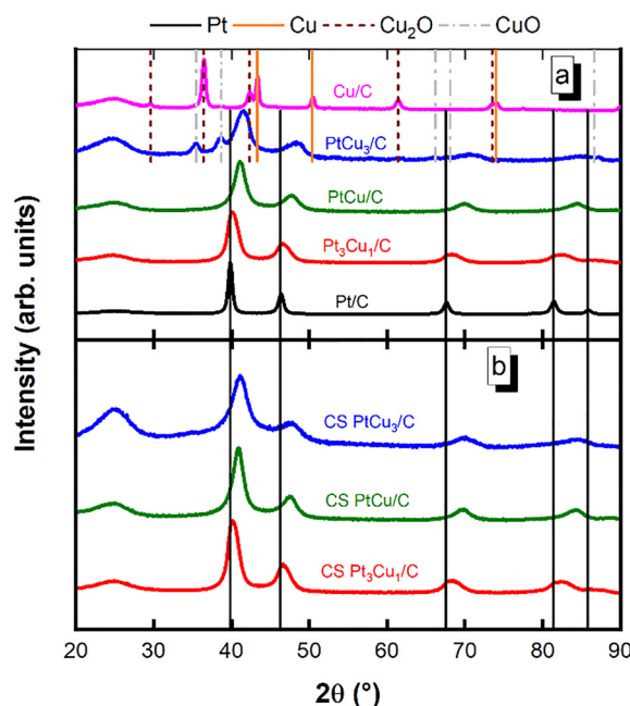
Fig. 2 Diffraction patterns of the prepared electrocatalysts: (a) base, and (b) CS (vertical lines and legends correspond to the XRD peaks of the different species present in the electrocatalysts).
