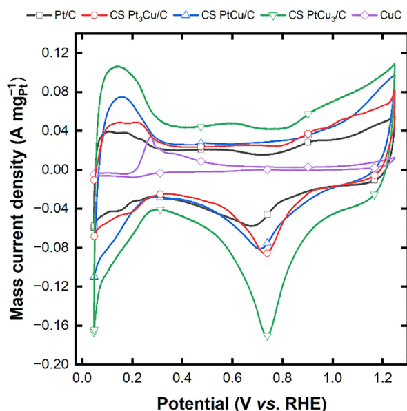
Fig. 5 Cyclic voltammetry (50 \text{mV s}^{-1} ) of the electrocatalysts in 0.5 mol \text{L}^{-1} \text{H}_2\text{SO}_4 .
