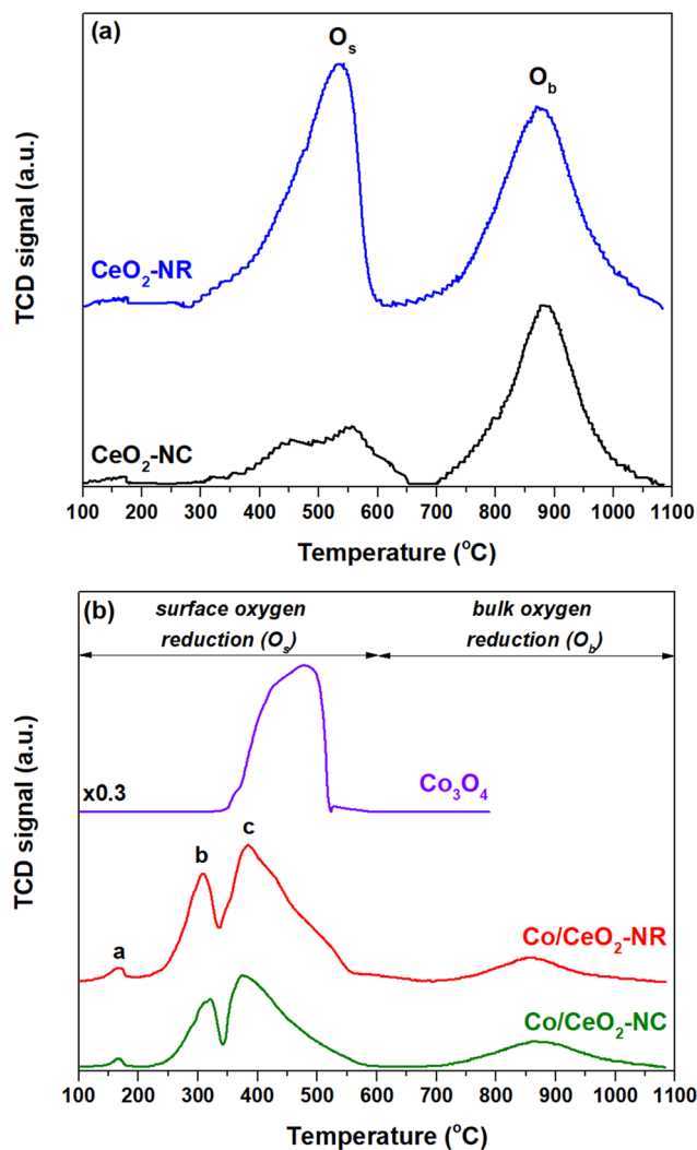
Fig. 7 H_2 -TPR profiles of (a) bare CeO_2 and (b) commercial Co_3O_4 and Co/CeO_2 samples.
