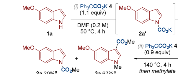
Scheme 2 Mechanistic investigation. a NMR yields using 1,1,2,2-tetrachloroethane as an internal standard.
