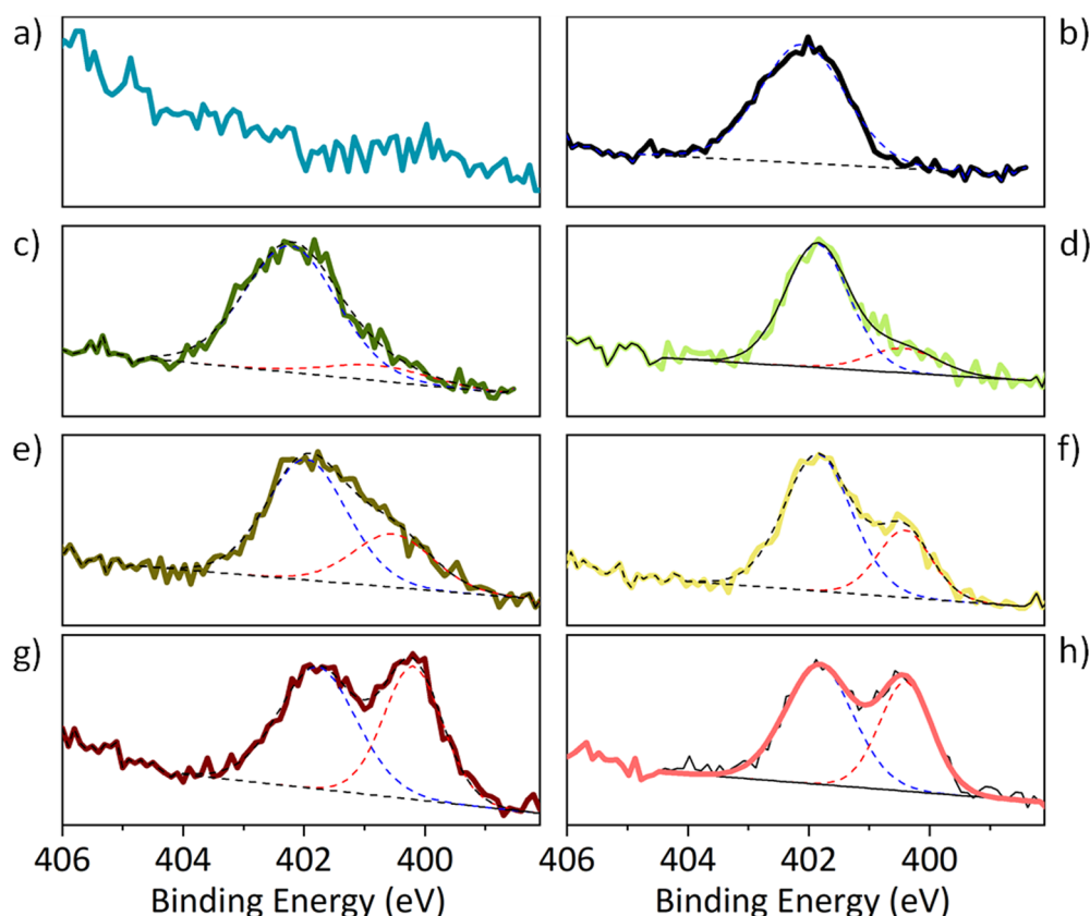
Fig. 8 Nitrogen 1s spectra curve fit into \text{NH}_2 (400.3 eV) and \text{C-NH}_2^+ (402.0 eV). (a) Cs-70, (b) PEA only, (c) FA 0.05 CS 0.95 -110, (d) FA 0.05 CS 0.95 -70, (e) FA 0.10 CS 0.90 -110, (f) FA 0.10 CS 0.90 -70, (g) FA 0.15 CS 0.85 -110, (h) FA 0.15 CS 0.85 -70.
