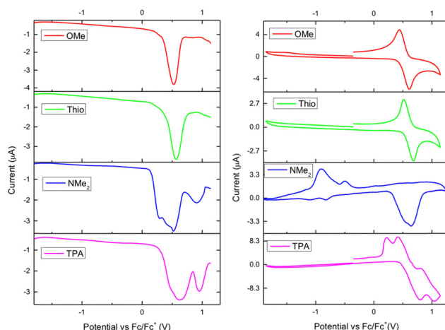
Fig. 7 Electrochemical analysis of all compounds (SWV left, CV right). All measurements were conducted at 5 \times 10^{-4} M -1 in \text{CH}_2\text{Cl}_2 with 0.1 M TBAPF 6 as the supporting electrolyte and ferrocene as an external standard.
