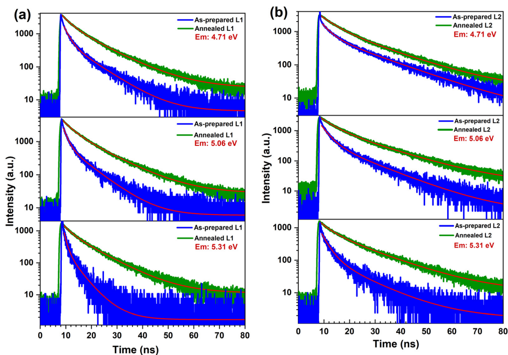
Fig. 10 Effect of annealing on the 4f 1 5d 1 → 3 H 4 , 3 H 5 , 3 H 6 luminescence decay of the \text{Pr}^{3+} ions for (a) L1 and (b) L2 nanocrystals, recorded under the intra-center excitation of the \text{Pr}^{3+} ion by the 6.54 eV photons at 7 K. Experimental data (green and blue lines) are fitted by the bi-exponential decay function, which is shown by red lines. The decay curves are normalized at their maxima for better comparison.
