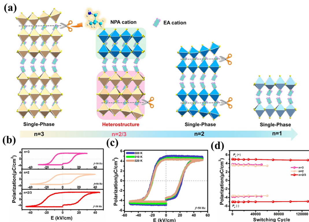
Fig. 6 (a) The figure illustrates self-assembling heterostructure (EA) 2 (EA) n-1 PbBr 3n+1 ( n = 2/3 ) and individuals n = 1 to 3 single crystal halide hybrid perovskites, (b) ferroelectric P - E hysteresis loops at 50 Hz, (c) the P - E loops of n = 2/3 heterostructures at different temperatures, and (d) the fatigue test for n = 2, n = 2/3, n = 3 . Reproduced from ref. 72 with permission from John Wiley and Sons, copyright 2025.
