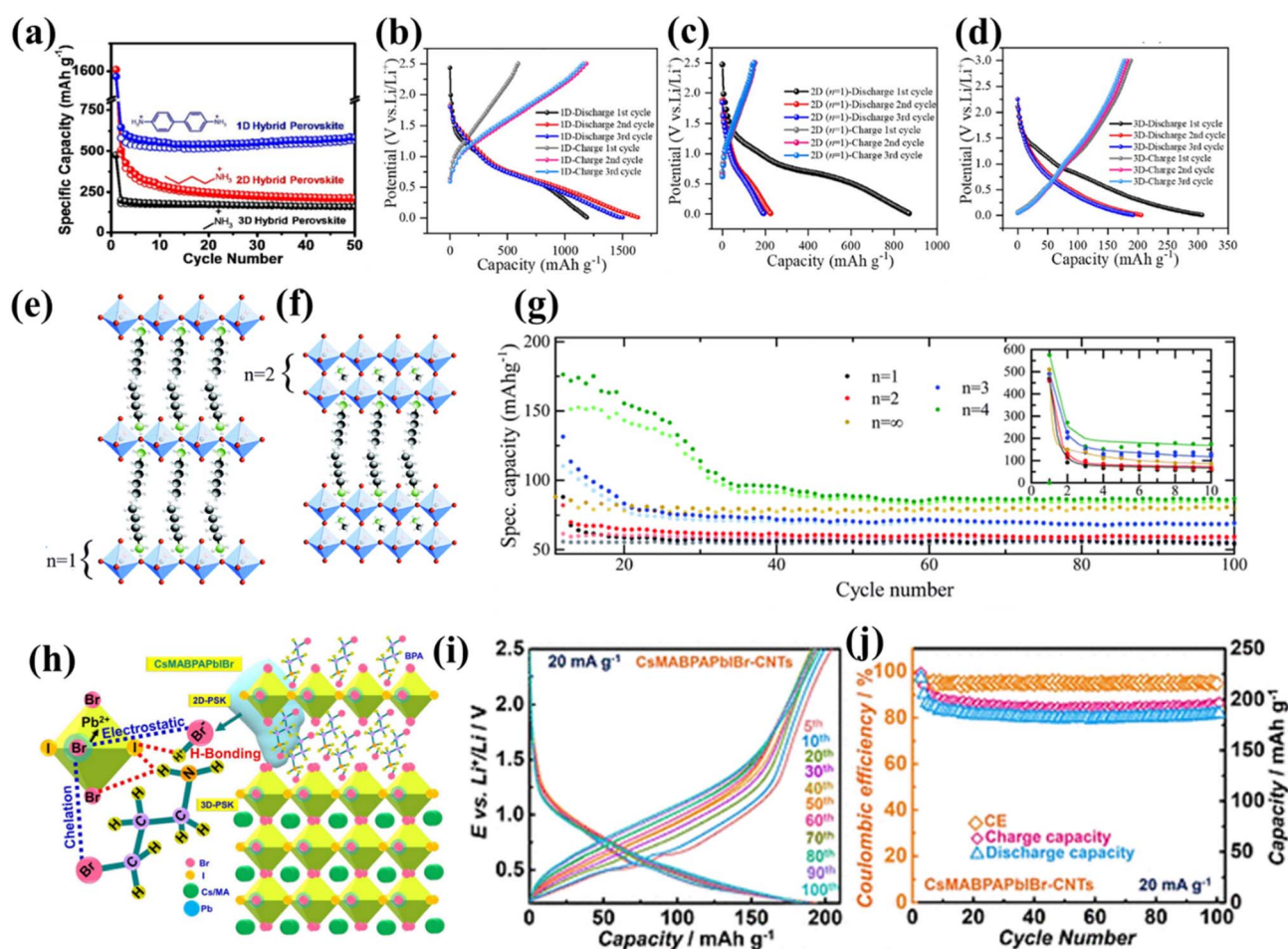
Fig. 10 (a) Cyclic stability for 1–2–3 D hybrid perovskite at a current density of 100 \text{ mA g}^{-1} in the potential window of 2.5 – 0.01 \text{ V} 172 Copyright 2017, J. Mater. Chem. A . Galvanostatic charge–discharge profiles of first three cycles of (b–d) 1D, 2D and 3D perovskite at a current density of 100 \text{ mA g}^{-1} between 0.01 and 2.50 \text{ V} 186 Copyright 2022, J. Energy Chem. (e) Quasi 2D (\text{BA})_2(\text{MA})_{n-1}\text{MnX}_{3n+1} ( n = 1 ) perovskite structure with individual layers of \text{PbX}_4 intercalated between two BA organic chains. (f) n = 2 -layered perovskite structure. (g) Gravimetric charge–discharge capacities of the bromide-based layered perovskite (\text{BA})_2(\text{MA})_{n-1}\text{Pb}_n\text{Br}_{3n+1} from n = 1 – n = 4 and the respective bulk \text{MAPbBr}_3 perovskite (equivalent in structure to n = \infty ) as a function of cycle number from cycle 11–100; the first 10 cycles are highlighted in inset. Specific charge capacities are shown shaded and specific discharge capacities block colour. A current density of 30 \text{ mA g}^{-1} and a potential window of 2.85 – 0.1 \text{ V} are used 180 Copyright 2021, Mater. Adv. (h) Schematic structure of 2D–3D hybrid PSK ( \text{CsMABPAPbI}_3 ), showing the interactions between \text{Br}(\text{Pr})\text{NH}_2 – \text{HBr} and the unit cell of the PSK (perovskite). (i) GCD plots acquired intermittently during cycling at 20 \text{ mA g}^{-1} , (j) capacity/CE variation with cycling 171 Copyright 2025, ACS Appl. Energy Mater.
