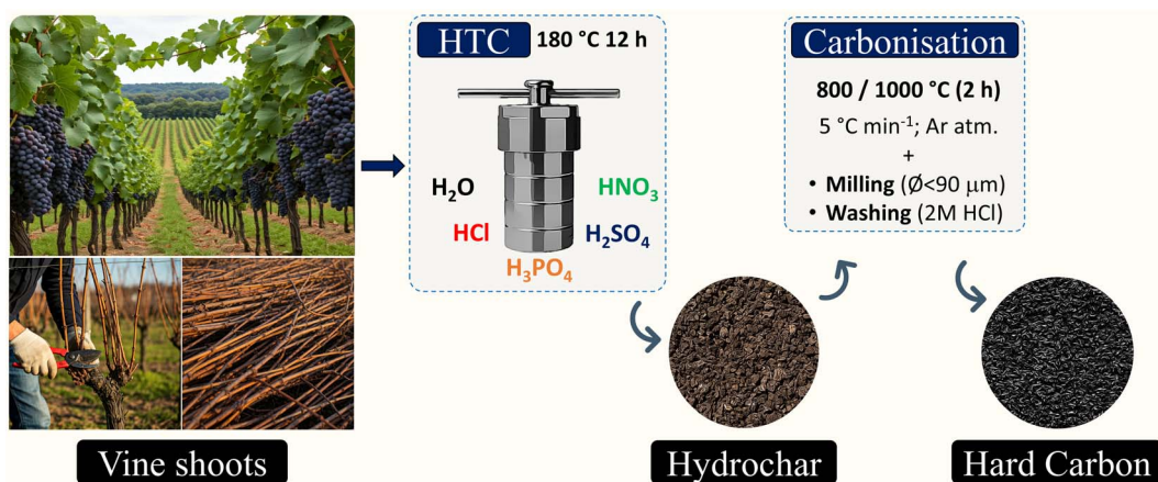
Fig. 1 Graphical summary of the hard carbon synthesis via HTC.
