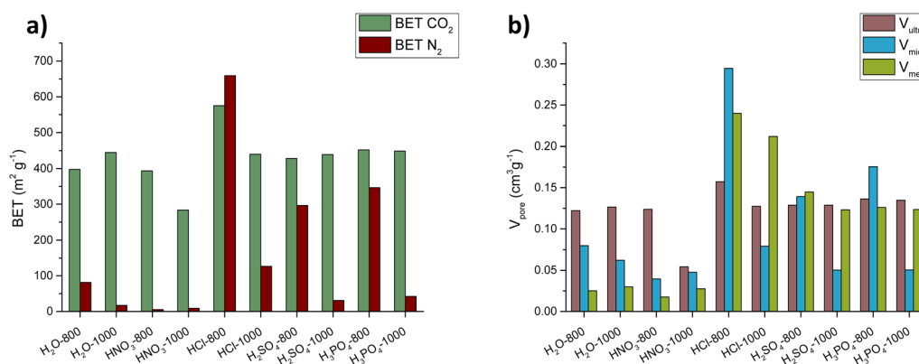
Fig. 3 (a) BET surface areas and (b) pore volumes for all the hard carbons under study.
