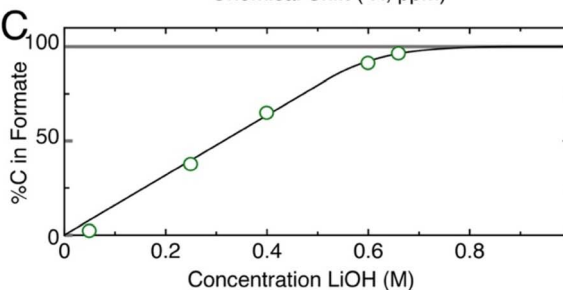
Fig. 3 Product concentration depending on (A) substrate concentration and (B and C) LiOH concentration. The line in (C) is a guide to the eye, and 0.6 M LiOH corresponds to 1 equiv. per substrate carbon. Reaction conditions: (A) variable and (B and C) 0.05 M cellobiose, (A) 0.6 M and (B and C) variable LiOH as indicated and 24 equiv. hydrogen peroxide in a 1.5 mL Eppendorf tube (200 \mu\text{L} \text{H}_2\text{O}/\text{D}_2\text{O} (90%/10%)) at 308 K, shaken at 600 rpm for 20 h.
