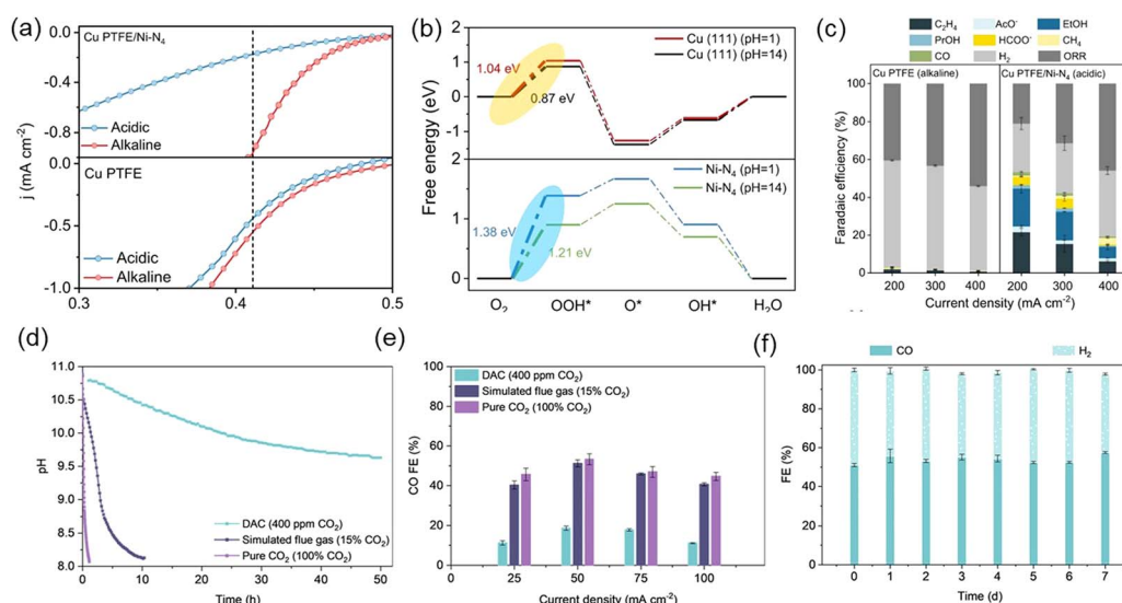
Fig. 7 (a) LSV curves in pure O 2 saturated acidic and alkaline electrolytes. (b) Free energy diagrams of ORR on Ni-N 4 and Cu PTFE at 1.23 V vs. SHE. (c) Product FE for Cu PTFE in 1 M KOH and Cu PTEE/Ni-N 4 in 0.05 M H 2 SO 4 + 1.5 M Cs 2 SO 4 under different current densities. (d) pH of a 2 M K-Gly with 0.1 M KH 2 PO 4 capture solution over time while capturing CO 2 from the atmosphere (400 ppm), CO 2 from a simulated flue gas (15%), and pure CO 2 (100%). (e) FE towards CO using the post-capture solutions of the capture processes in (d). (f) FE towards CO and H 2 of a newly assembled electrolyzer while continuously operating at 50 mA cm -2 and exposing the same capture solution to 100 sccm of air for 7 days. (a–c) Reproduced with permission. 54 Copyright 2024, Springer. (d–f) Reproduced with permission. 55 Copyright 2024, Springer.
