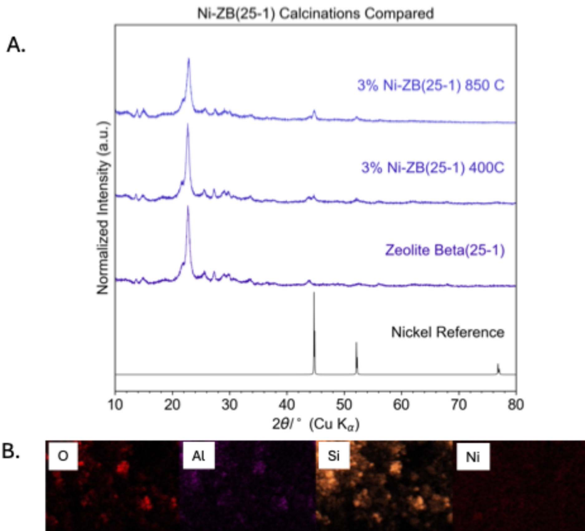
Fig. 9 (A) XRD patterns of 3%Ni-ZB(25 : 1) calcined at 400 °C and 850 °C. (B) EDS mapping of 3%Ni-ZB(25 : 1) calcined at 850 °C.
