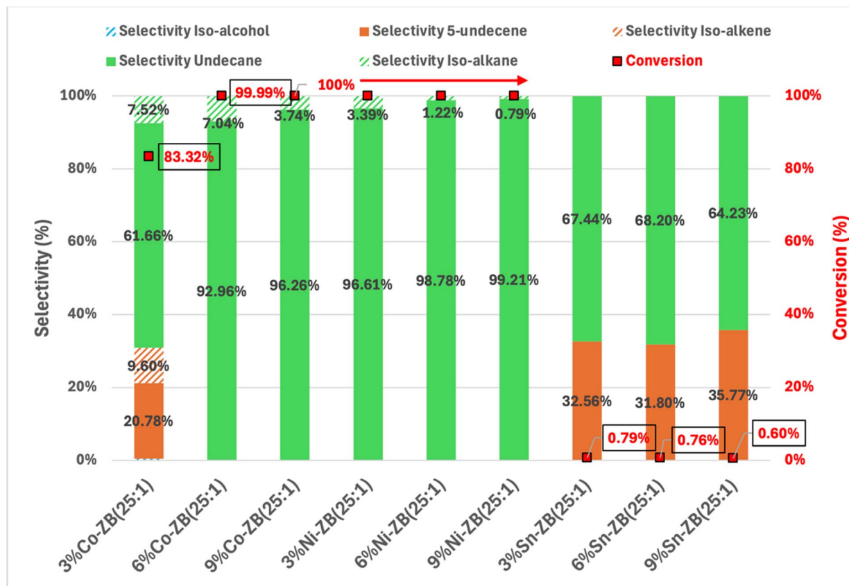
Fig. 11 Conversion and selectivity of all ZB(25 : 1) catalysts. Green = undecane and isomers associated. Orange = undecene and isomers associated. Blue = 6-undecanol and isomers associated.
