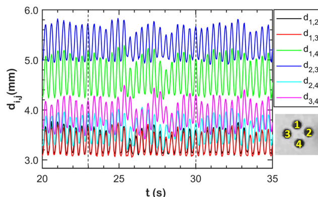
Fig. 6 Dynamics of four small motors: distance between beads i and j ( d_{ij} ) as a function of time. The dashed lines at t = 23 \text{ s} and 30 \text{ s} indicate that the oscillations of the beads are in phase. Field of view of grayscale image is 11 \text{ mm} \times 10 \text{ mm} .
