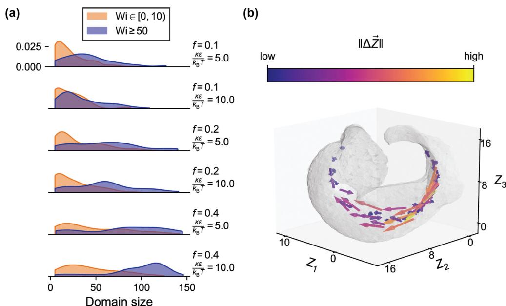
Fig. 8 Examination of shear-induced changes to morphology at quiescent conditions. (a) Observed distributions of SCNP topological domain sizes for selected linker fraction f and stiffness parameters \frac{KE}{k_B T} ; all chains have N = 150 beads. Low Weissenberg number ( Wi < 10 ) is shown in orange; high ( Wi \geq 50 ) in blue. Y-Axis bounds are consistent across all plots. (b) Representative sampling of displacement of embedding-space centroids between SCNPs cross-linked at Wi = 0 and at the maximum simulated Wi for each parameter set. Arrows originate at the Wi = 0 centroids and point to the high- Wi centroids. Color encodes the displacement magnitude as another guide to the eye.
